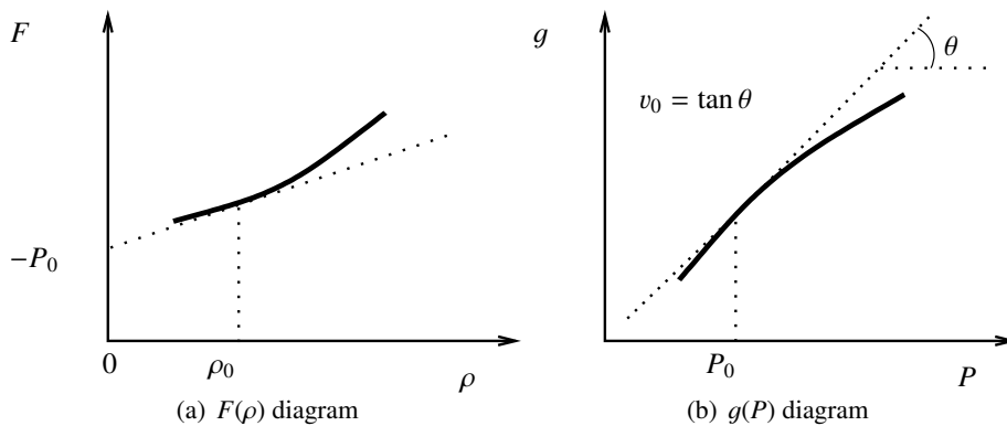
Figure 3.1: Main thermodynamic potentials for an isothermal fluid
