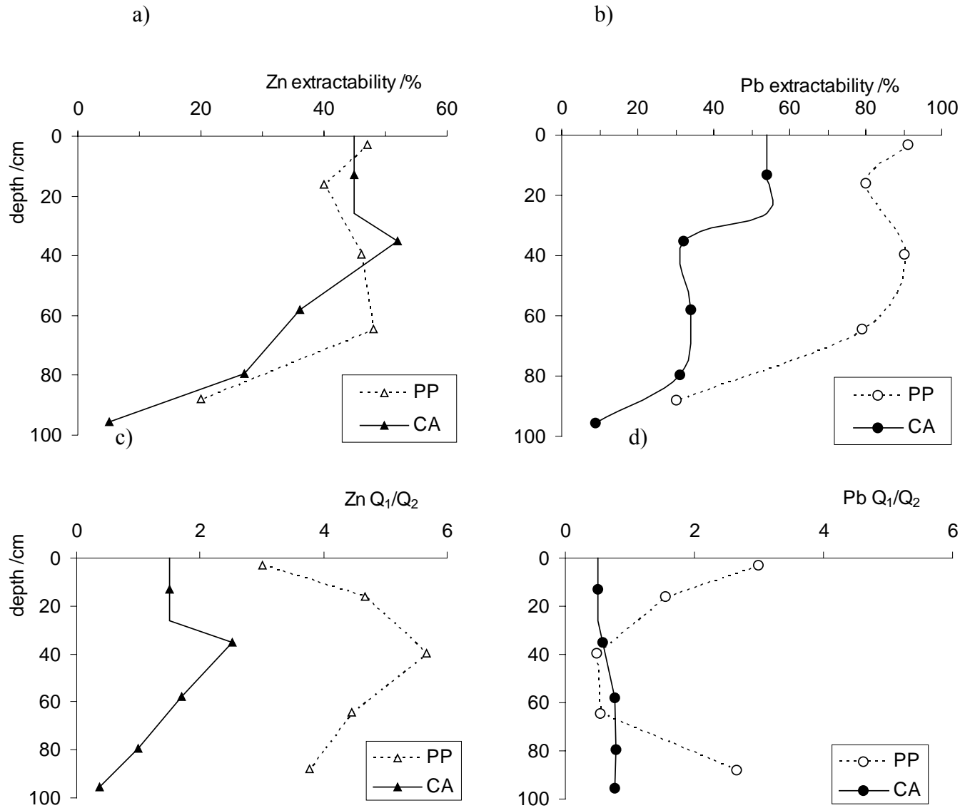
Figure 5.6. Concentrations of total EDTA extractable Zn and Pb (a, b) and ratios of readily Labile ( Q_1 ) and Less Labile ( Q_2 ) Zn and Pb (c, d) in different soil horizons of the PP and CA soils. \Delta : Zn in PP, \blacktriangle : Zn in CA, \circ : Pb in PP, \bullet : Pb in CA
