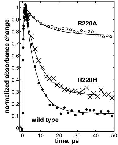
FIGURE 3: Kinetics at 442 nm of oxygenated FixLH: wild type (●), R220A (○), and R220H (×). Lines represent the global exponential fits of the data.
