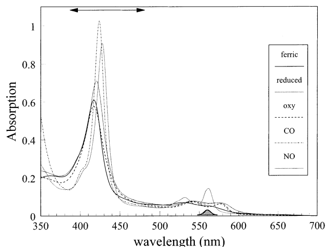
FIGURE 1: Ground-state absorption spectra of the different forms of DosH used in this study. The spectra are normalized to the same concentration. The spectral profile of the pump pulse and the probe region in the transient absorption experiments are indicated by the shaded area at the bottom and the bisided arrow, respectively.
