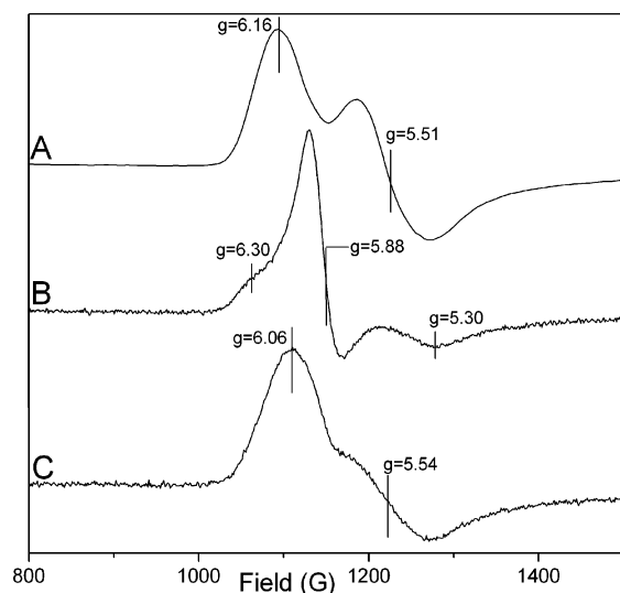
FIGURE 3: EPR spectra recorded for BjFixLH WT pH 7.45 (A), R220H pH 7.45 (B), and R220H pH 4.4 (C). Sample concentration: 50 \mu M, temperature 15 K. Samples were prepared in a 100 mM Hepes buffer for pH 7.45, and a 100 mM acetate buffer for pH 4.4.
