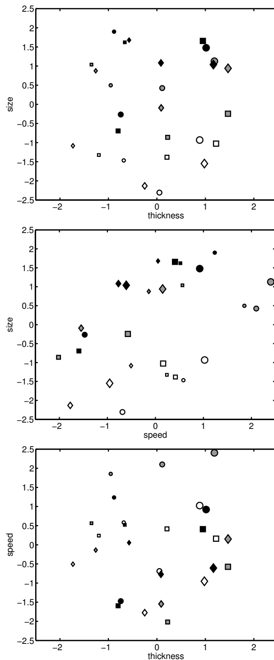
FIGURE 8.3: The three plots represent the perceptual space of the sounds after applying the basis transformation. The axes of the constructed three-dimensional space now indicate the mechanical parameters that have the highest correlations with these axes. In all three panels one of the three dimensions of the MDS analysis is perpendicular to the paper, so we can see only the two remaining dimensions. The mechanical properties of the plate are represented in the symbols. The size of the symbols represents the thickness of the plate, where the largest symbol corresponds to the thickest plate. The type of the symbol represents the speed of the ball. The circle was the slowest, the square the middle and the diamond the fastest. The fill color of the symbol represents the size of the rolling ball, with the open symbol representing the small ball, the grey one the middle and the black ones the largest balls.
