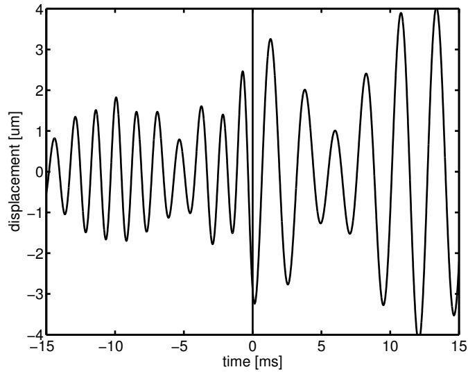
FIGURE 6.8: The plate vibrations at a fixed point vary in frequency due to the Doppler effect. The example shown is obtained for a 500 Hz sinusoidal imposed force moving with a speed of 500 m/s. The origin of time corresponds at the very instant where the source passes at the fixed point. At the left side where the source approaches the observation point, the average frequency is 638 Hz, and it is 419 Hz at the right side.
