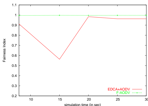
Figure 5.5: Fairness Index
