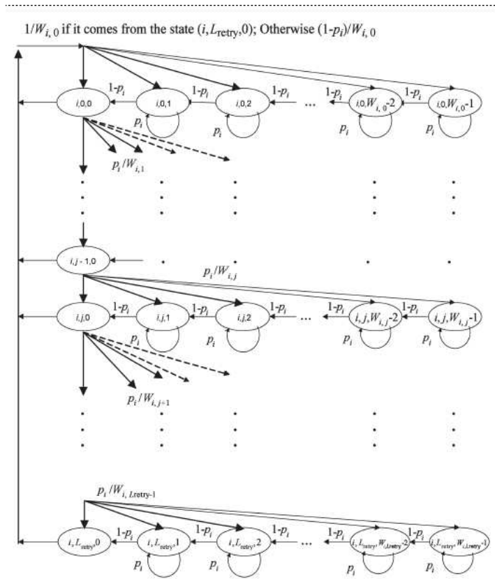
Figure 3.3: Markov chain
