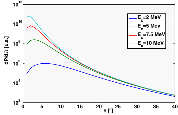
Figure 5.17: Angular distribution of the Bremsstrahlung emission for different electron energies.
