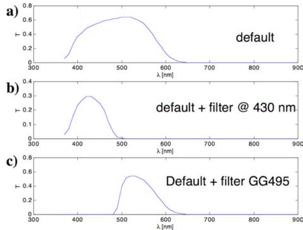
Figure 6.6: a) Transmission of common optical element. b) Transmission of common optical element using the 430 nm filter. c) Transmission of common optical element using the GG495 filter.
