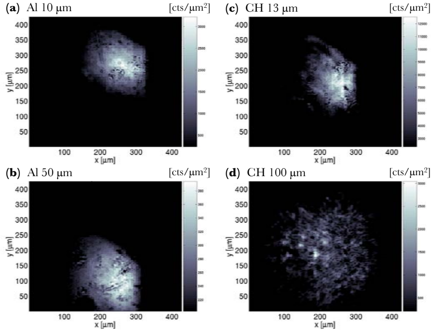
Figure 6.11: Optical emission (counts/ \mu\text{m}^2 ) images obtained using 10 and 50 \mu\text{m} Al [(a), (b)] and 13, 100 \mu\text{m} CH targets [(c), (d)].
