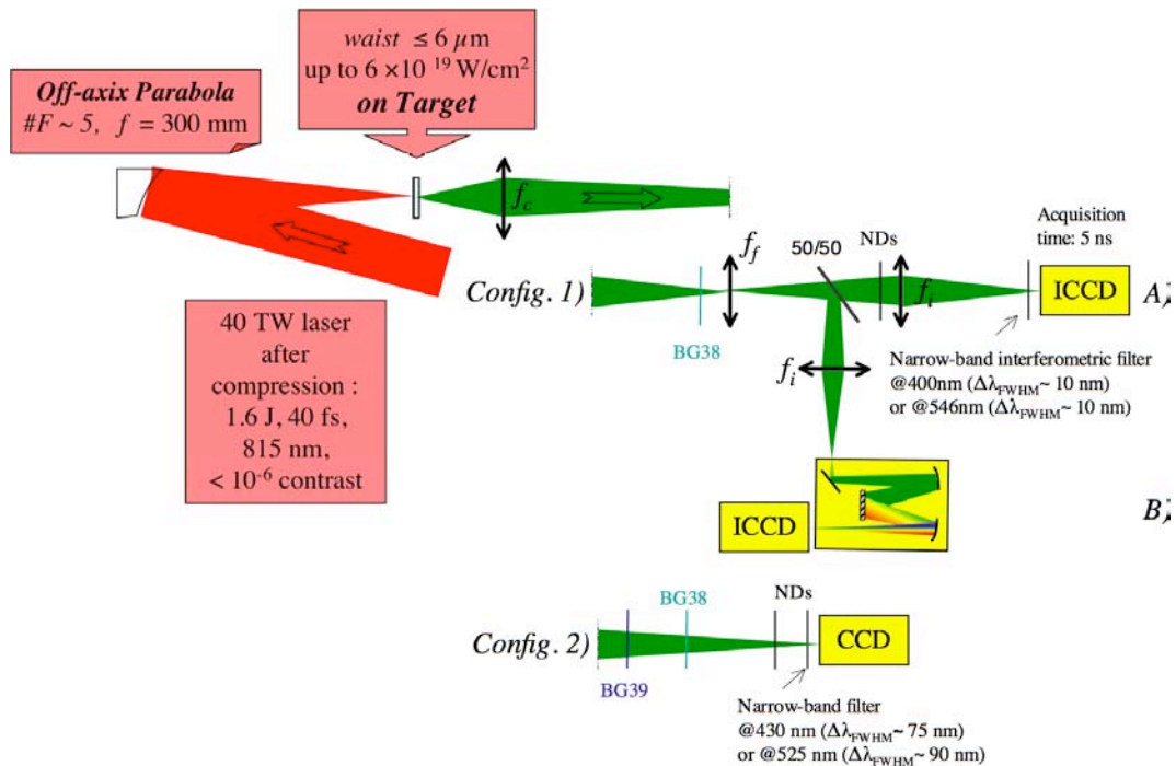
Figure 12.1: Installation expérimentale.
