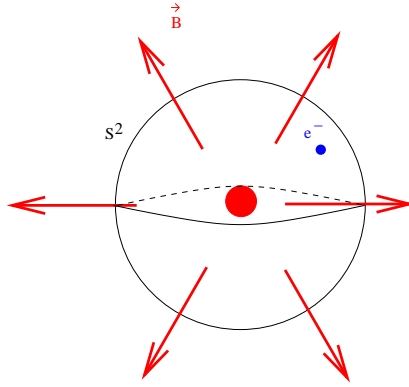
Figure 15: An electron bound to a sphere, with a magnetic monopole in the middle of the sphere.
