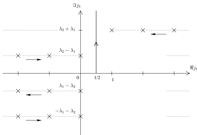
Figure 10: Integration contour and poles for the operator product expansion of a degenerate field and a non-degenerate field. The dotted lines indicate the poles, and the arrows indicate in which direction the poles move when \lambda_1 acquires an increasing imaginary part.
