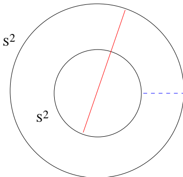
Figure 19: A (blue dashed) string of minimal length and a (red) string of maximal length, stretching between two su(2) orbits.
