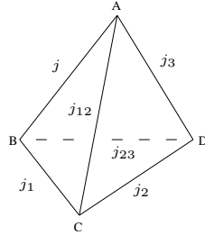
Figure 21: The 6j symbol as a tetrahedron.
