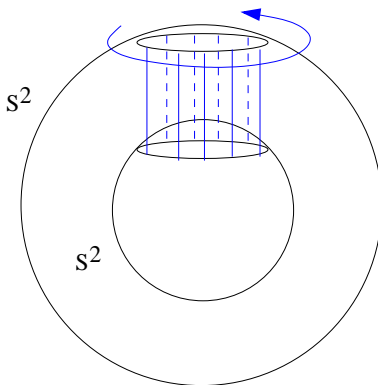
Figure 17: A rigid string stretching between two different su(2) orbits, and rotating.
