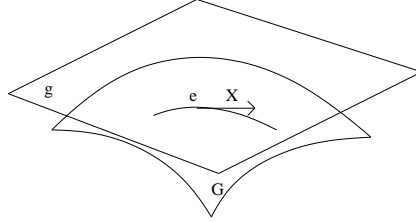
Figure 4: Relation between a Lie group G and its Lie algebra \mathfrak{g} . The point e is a point on the group (say, the identity) and X is the tangent vector at this point of the left-invariant vector field pictured here as a curve on the group manifold G .
