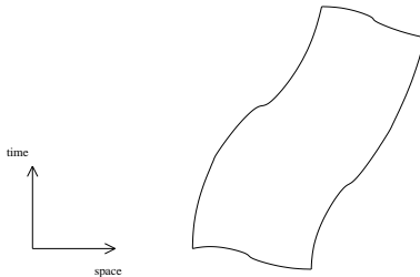
Figure 2: The string worldsheet is the two-dimensional surface in space-time which represents the evolution of the string in the course of time.
