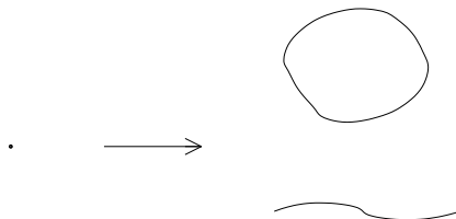
Figure 1: The fundamental idea of string theory is to replace points by (closed or open) strings.
