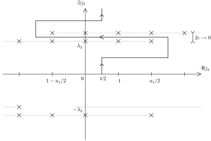
Figure 11: Integration contour and poles for the operator product expansion of a degenerate field and a non-degenerate field.
