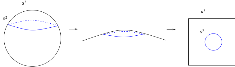
Figure 18: The limit turning a conjugacy class into an orbit for the example of G = SU(2) . The size of the conjugacy class (orbit) is kept fixed, while rescaling the group metric until it becomes flat.
