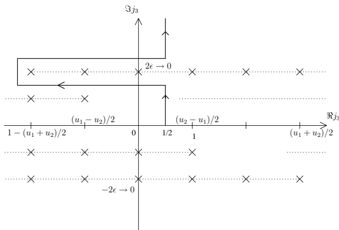
Figure 12: Integration contour and poles for the operator product expansion of two degenerate fields.
