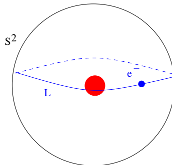
Figure 16: The (blue) curve traced by the electron associated to a Wilson loop. The Wilson loop can be computed by calculating the flux through the upper cap (– the hat –) or the lower cap (– the bowl –), and must be unambiguous.
