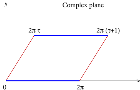
Figure 8: The torus as a Riemann surface. Periodicity conditions on the torus are imposed by identifying (thick) blue lines and (thin) red lines respectively.
