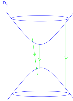
Figure 24: Some past time-like strings starting on a future discrete orbit and ending on a past discrete orbit.
