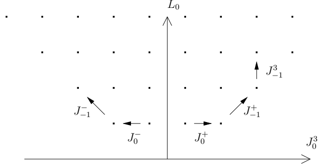
Figure 9: A degenerate representation of the affine Lie algebra \widehat{sl(2, \mathbb{R})}_{k+2} , built from a finite representation of the Lie algebra sl(2, \mathbb{R}) . Each dot indicates a state in the representation. Arrows indicate how the currents act on these states.
