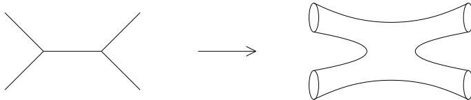
Figure 3: Feynman diagrams of particle physics are replaced by smoother equivalents in string theory. An example is pictured above for four closed strings. The interaction does not happen at any specific point anymore.
