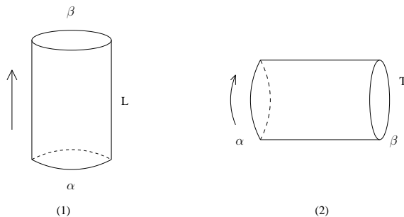
Figure 7: Two ways of calculating the partition function Z_{\alpha\beta} : (1) on the cylinder, between the boundary states |\alpha\rangle and |\beta\rangle , (2) as a periodic time evolution on the strip, with boundary conditions \alpha and \beta .
