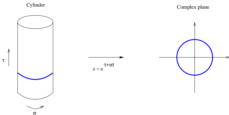
Figure 5: The cylinder is conformally mapped to the complex plane, therefore leading to radial quantization. A constant time line is pictured in thick blue.
