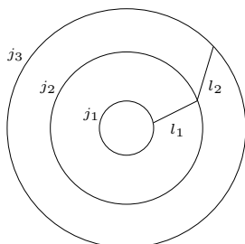
Figure 22: Two strings interacting.
