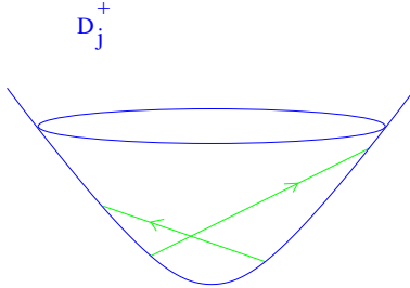
Figure 25: A few space-like strings starting and ending on a given discrete orbit.
