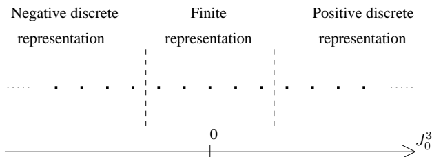
Figure 13: A continuous representation of the zero modes (or Lie algebra) of SL(2, \mathbb{R}) . Each dot corresponds to a state. The figure shows how a continuous representation decomposes into the sum of two (conjugate) discrete representations and of a finite representation, sandwiched by the discrete representations. These states play the role of primary states of the associated affine Lie algebra representation.
