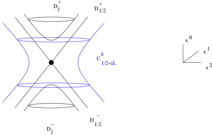
Figure 23: The sl(2, \mathbb{R}) co-adjoint orbits. One-sheeted hyperboloids correspond to continuous representations and two-sheeted hyperboloids to discrete representations (the upper sheet being associated to positive discrete representations and the lower sheet to negative ones). The future and past light-cone (with the point at the origin removed) correspond to the special cases of discrete representations with j = \frac{1}{2} while the point at the origin represents the trivial (identity) representation.
