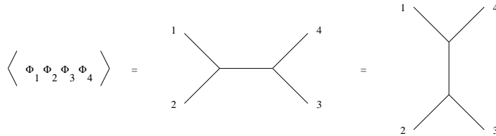
Figure 6: Crossing symmetry.
