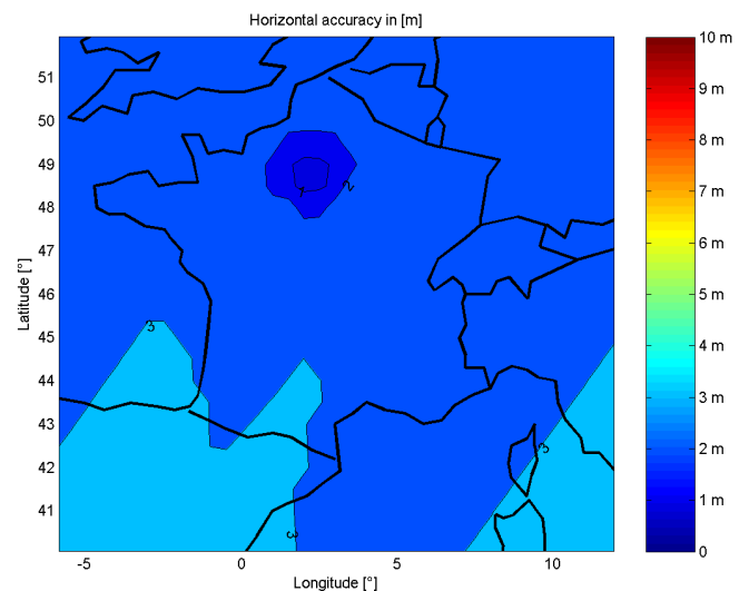
Figure 2.20: Positioning server accuracy.
