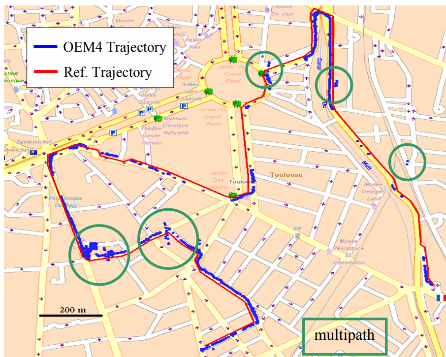
Figure 6.9: Reference trajectory (red) and OEM4 position solution (blue). Urban trial.
