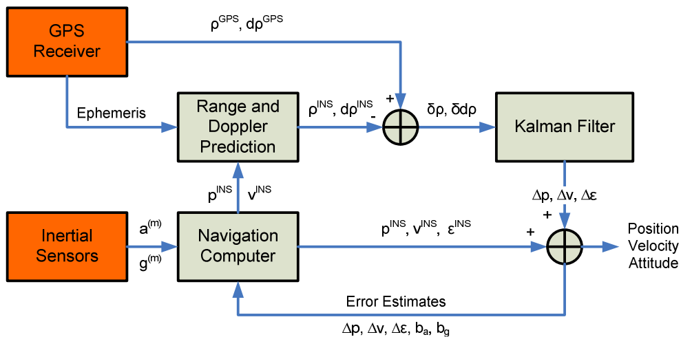
Figure 6.4: Tight coupling integration scheme. Closed-loop architecture.
