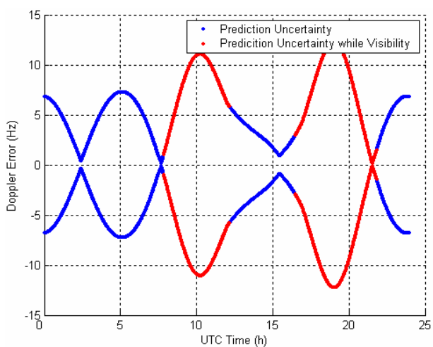
Figure 5.5: Satellite Doppler uncertainty. GPS time known at \pm 2s . User's position uncertainty of \pm 15km .
