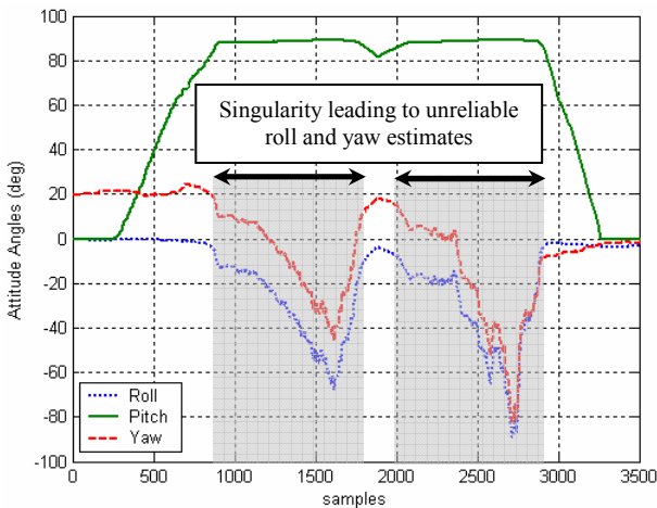
Figure 3.6: Euler's angles singularity issue.
