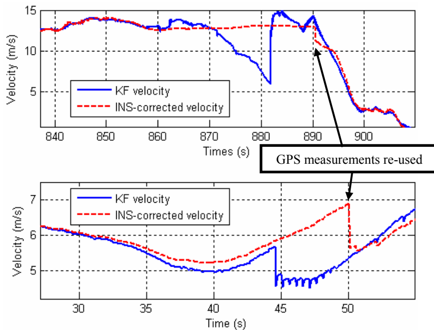
Figure 6.17: Along track velocity profile corrected by the Inertial Navigation System when bad satellites configurations are detected.
