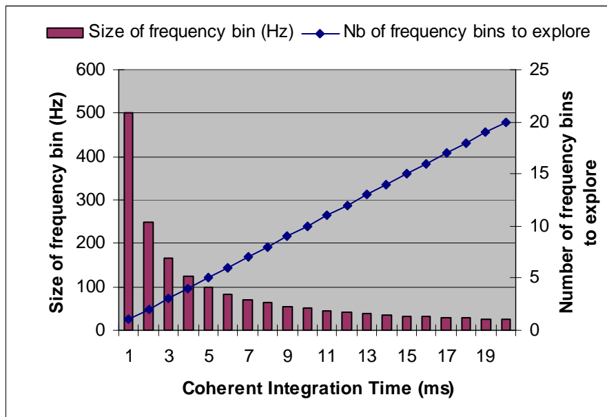
Figure 5.8: Frequency bins and number of frequency bins to explore with respect to a user Doppler uncertainty of \pm 250 Hz.
