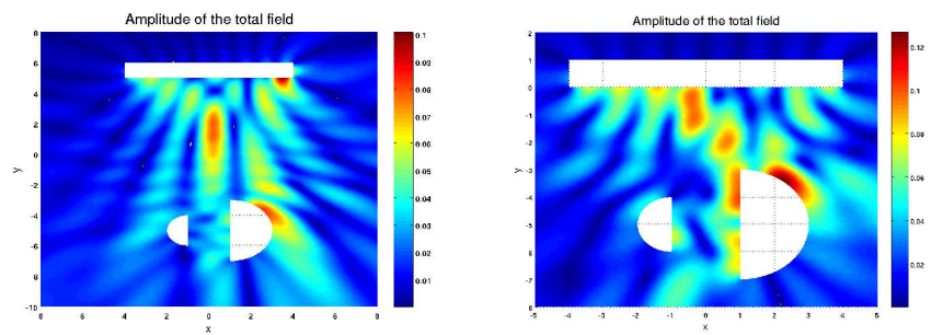
FIG. 2.5 – Emission of the third eigenvector for k = 3.14 (left : D = 8 , right : D = 3 ).
