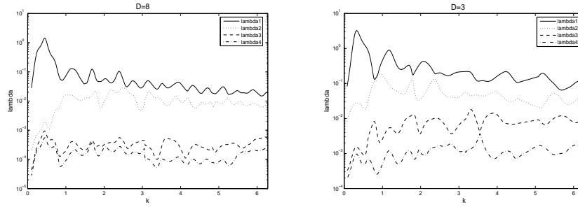
FIG. 2.10 – First model : 4 largest eigenvalues of T according to k .
