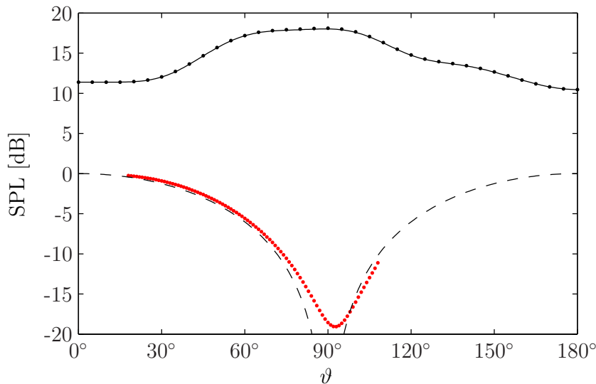
Figure 5.11: Acoustic directivity D(\vartheta) as found from the DNS (●), compared to a dipole D(\vartheta) \propto \cos \vartheta (dashed line). Prediction from the Lighthill equation with (●) and without (—) assumption of radially compact sources.
