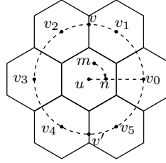
Figure 13.6: Level 1
