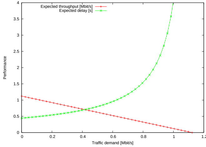
Figure 10.1: Expected throughput and delay for DSCH.
