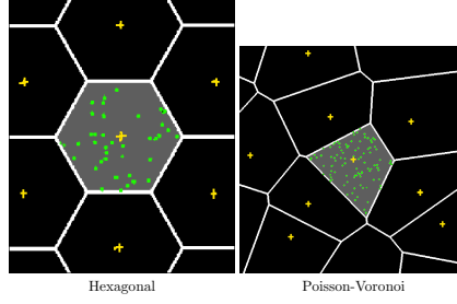
Figure 2.2: Hexagonal and Poisson-Voronoi models
