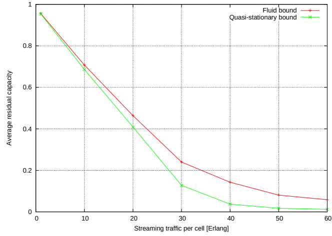
Figure 10.13: Comparison of fluid and quasi-stationary bounds.
