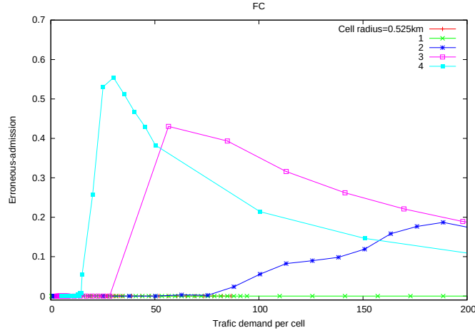
Figure 13.18: FC erroneous-admission
