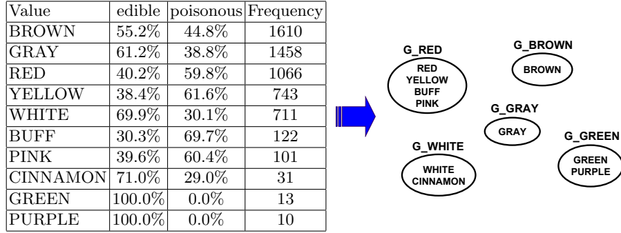
Fig. 3. MODL grouping of the values of the Cap Color variable for the classification of the Mushroom dataset in 2 classes
