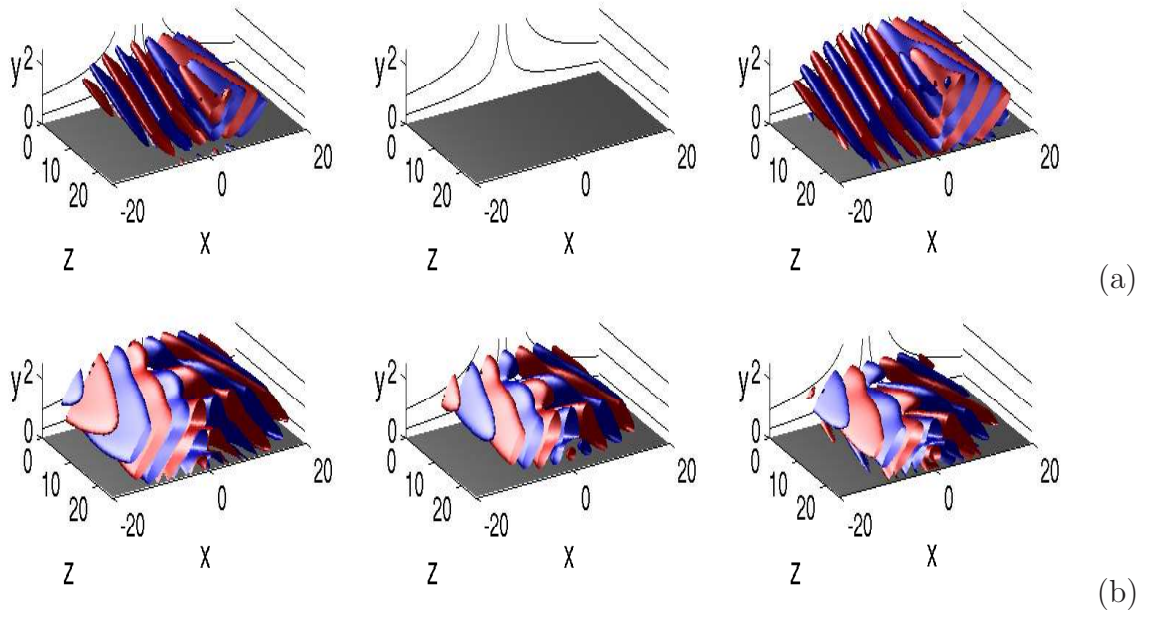
Figure 3.7: From left to right, chordwise, wall-normal and spanwise vorticity components of k = 0.25 optimal perturbations at t = 0 (a) and at maximum amplification time T = 72 (b). The isosurfaces correspond to 0.1 (red) and -0.1 (blue) times the maximum of the strongest vorticity component. At t = 0 the vorticity maxima are \omega_{x0} = 0.31 , \omega_{y0} = 0.01 , \omega_{z0} = 1 , and at t = T , \omega_{xT} = 9.4 , \omega_{yT} = 3.9 , \omega_{zT} = 3.3 . The Reynolds number is Re = 550 .
