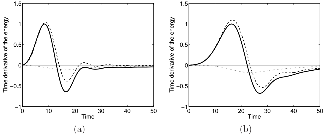
Figure 2.5: Temporal evolution of the dominant terms in the energy equation (2.44) for optimal perturbations, integrated over the (y, z) -plane and normalized with respect to the maximum time derivative of the energy. The production term -ReW'wv (dashed line) is responsible for most of the energy amplification (solid line). The dissipation term w\Delta w is displayed as a dotted line. Parameter settings are (a) Re = 2000, k = 0.1, T_p = 12.9 and (b) Re = 2000, k = 0.4, T_p = 22.2 .
