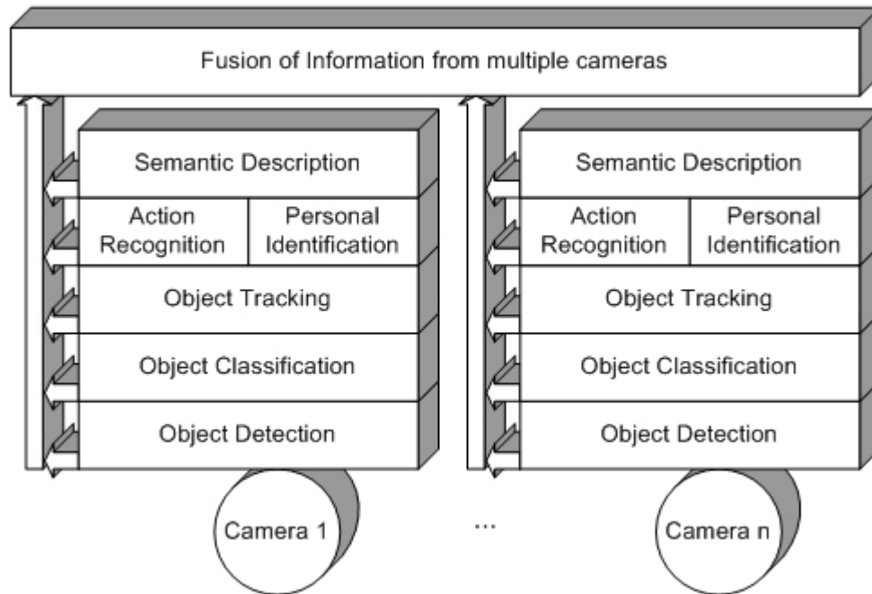
Figure 4.1: A generic framework for intelligent visual surveillance
