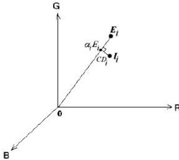
Figure 5.9: Proposed color model in three dimensional RGB color space
