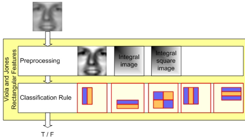
Figure 6.5: Viola and Jones rectangular features
