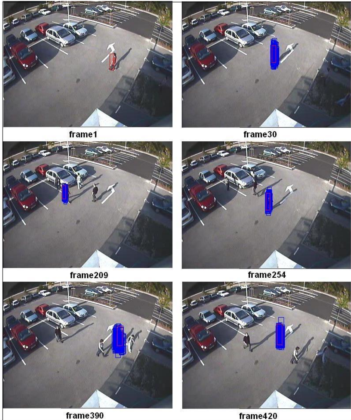
Figure 7.1: Tracking results with displaying all particles
