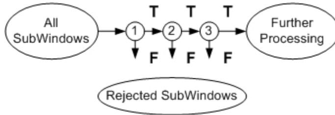
Figure 6.16: Attentional cascade of classifiers
