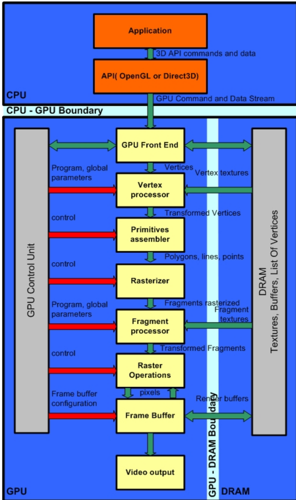
Figure 8.5: Graphics pipeline
