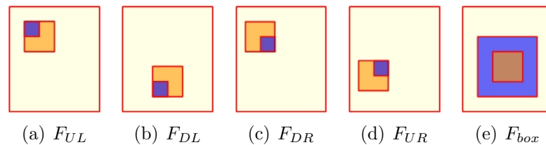
Figure 6.14: Classification rules used within extended rectangular features
