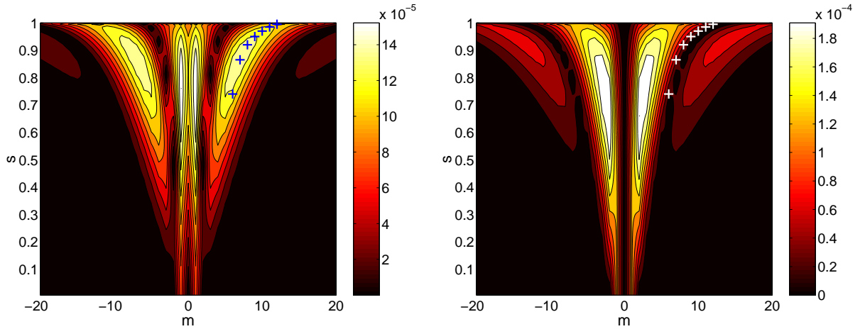
Figure 3.3: Spectrum of 2|\tilde{b}_{m,-3}^1| (dimensionless quantity) as a function of m and the radial coordinate s , for 1kAt in the I-coils, with crosses showing the position of the resonant harmonics, \tilde{b}_{res}^1 . Left: even parity configuration. Right: odd parity configuration.
