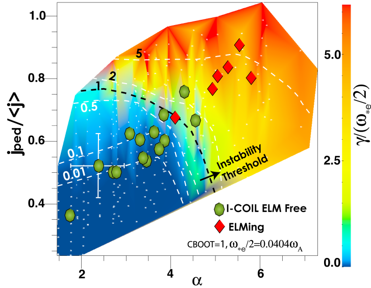
Figure 2.6: Position of the plasma in a diagram showing, as a function of the normalized radial pressure gradient ( \alpha ) in the pedestal and normalized toroidal current density in the pedestal ( \langle j_{ped}/\langle j \rangle ), the growth rate of the most unstable peeling-ballooning mode ( \gamma ) normalized to half the electron diamagnetic drift frequency ( \omega_{*e} -see footnote for an explanation). Taken from [36].
