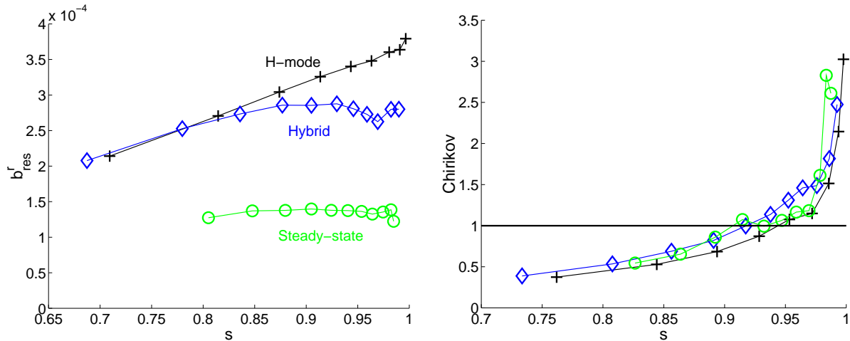
Figure 5.8: Crosses: profiles of b^r_{res} (left) and \sigma_{Chir} (right) for the design with two rows of eighteen external coils fed with 400kAt (diamonds [resp. circles] correspond to a hybrid-like [resp. steady-state-like] q profile, see section 5.6).
