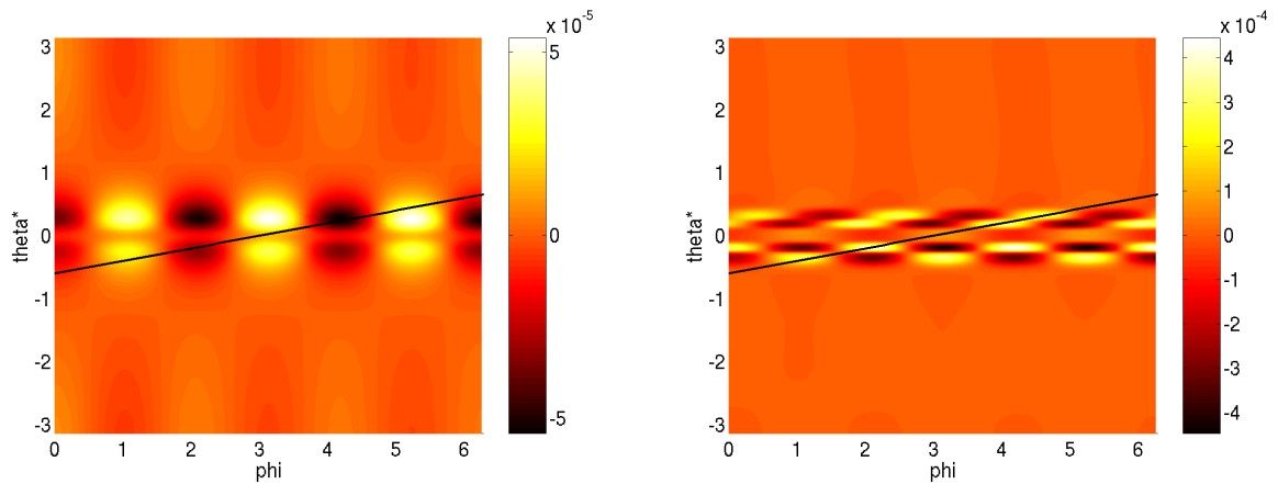
Figure 5.31: Colour plots of the normalized radial magnetic perturbations b^r on the s = 0.95 surface as a function of \varphi and \theta^* , together with a q = 5 field line, produced by the two rows of eighteen external coils (left) and the blanket coils with optimized phasing for q_{95} = 5 (right), for 1kAt.
