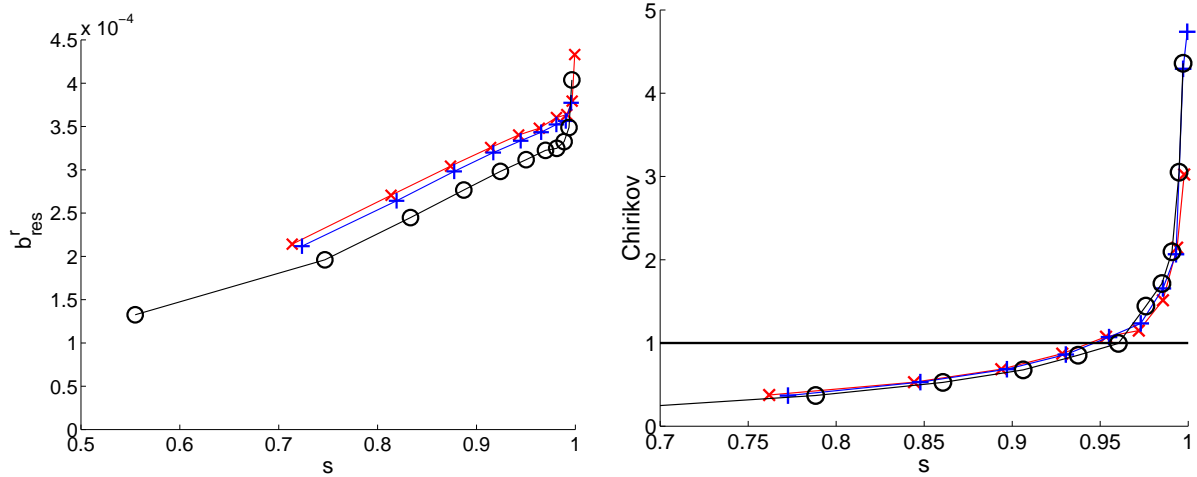
Figure 5.32: Profiles of b_{res}^r (left) and \sigma_{Chirikov} (right) for the two rows of eighteen external coils fed with 400kAt, with variations in \beta_p and l_i : red x's for \beta_p \simeq 0.64 and l_i \simeq 0.8 , black circles for \beta_p \simeq 0.6 and l_i \simeq 1 , and blue +s for \beta_p \simeq 1.2 and l_i \simeq 0.8 .
