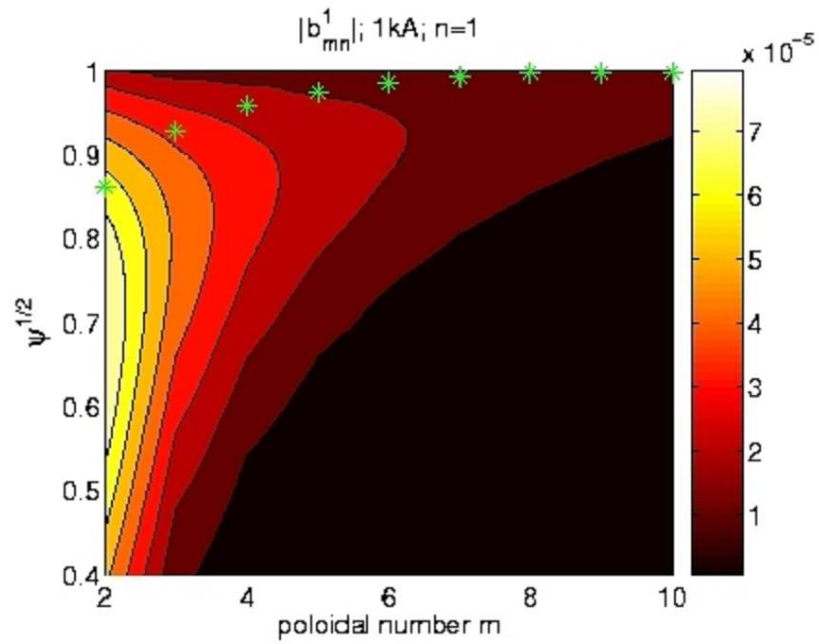
Figure 4.17: Spectrum of |b_{m,1}^1| (dimensionless quantity) as a function of the poloidal mode number and the radial coordinate for 1kAt in the EFCCs in n = 1 configuration, with stars showing the position of the resonant harmonics.
