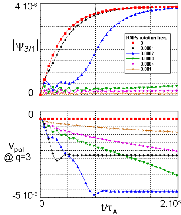
Figure 6.16: Temporal evolution of |\psi_{3/1}| and v_{pol} on the q = 3 surface for different values of \omega and a fixed \psi_{3/1}^0 = 10^{-5} .
