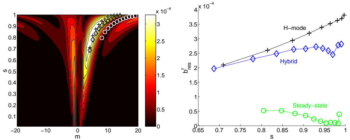
Figure 5.22: Top: same as fig. 5.20 but for the “optimized phasing” (0/-3/+3/0) configuration. Bottom: corresponding profile of b_{res}^r for 21kAt in the coils (diamonds [resp. circles] correspond to a hybrid-like [resp. steady-state-like] q profile, see section 5.6).
