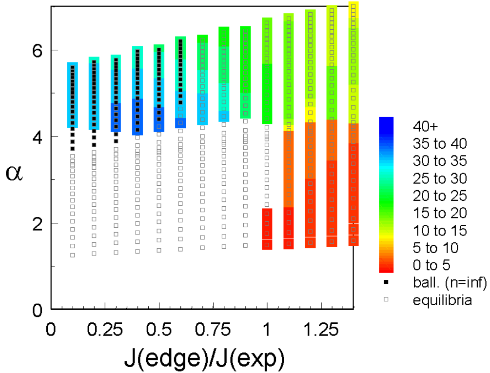
Figure 1.9: Example of the MHD P-B stability as a function of the normalized radial pressure gradient in the pedestal ( \alpha ) and the current density in the pedestal normalized to its experimental value for a JET H-mode discharge. Each square marks an equilibrium for which the stability was evaluated. The small black squares indicate instability of n = \infty ( n being the toroidal mode number of the mode - and n = \infty thus corresponding to modes infinitely localized perpendicularly to the equilibrium magnetic field) ballooning modes while the large coloured squares indicate instabilities with a finite n , the colour depending on the value of n . From [15].
