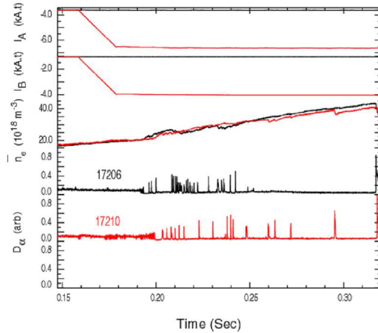
Figure 4.19: Comparison between a reference shot (17206, black traces) and a shot with the EFCCs in n = 1 configuration fed with 3kAt (17210, red traces). The traces represent, from top to bottom, the current in EFCCs A (two of the four EFCCs), the current in EFCCs B (the other two), the line-integrated electron density (which rises all along the discharge, a typical feature of MAST), and the D_\alpha traces for the two shots. (courtesy A. Kirk)
