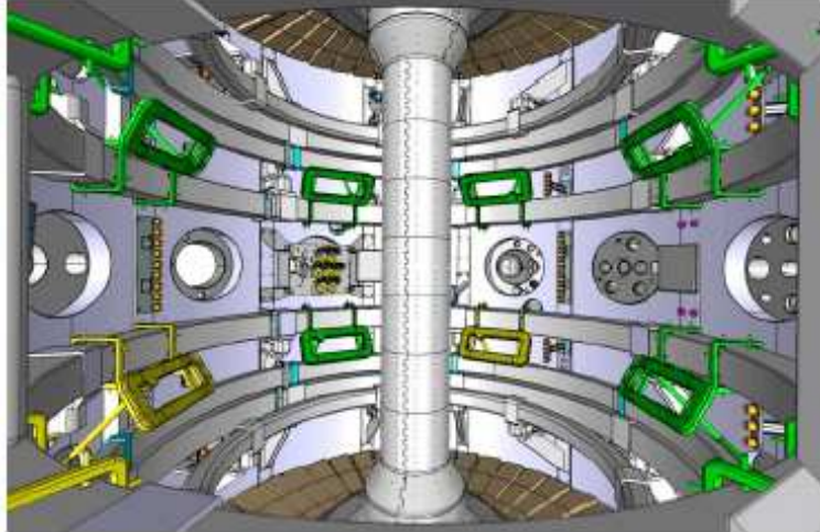
Figure 4.1: Design of the future ELMS control coils at MAST. (courtesy A. Kirk)
