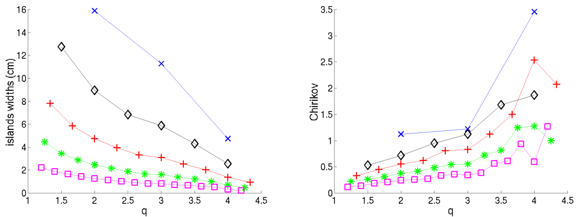
Figure 5.3: Islands widths and Chirikov parameter profiles for the compared designs ( q is used as a radial coordinate). Blue x's: n = 1 ; black diamonds: n = 2 ; red +'s: n = 3 ; green stars: n = 4 ; magenta squares: n = 5 .
