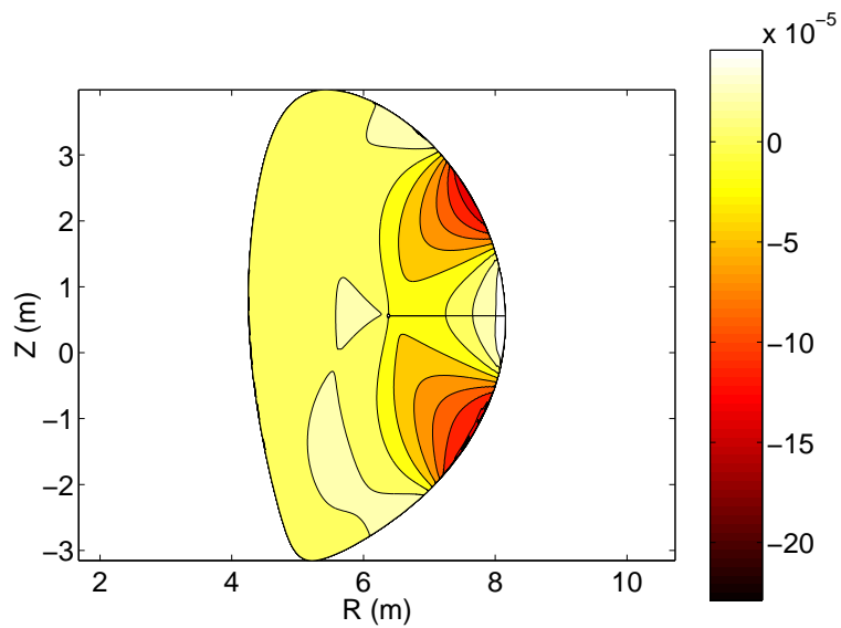
Figure 5.18: Poloidal cut of the normalized radial magnetic perturbation b' produced by the coils wound around the blanket modules, in 0/0/0/0 configuration, fed with 1kAt.
