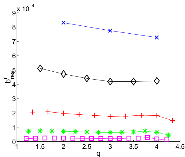
Figure 5.4: Profile of b_{res}^r (dimensionless quantity) for the compared designs ( q is used as a radial coordinate). Blue x's: n = 1 ; black diamonds: n = 2 ; red +'s: n = 3 ; green stars: n = 4 ; magenta squares: n = 5 .
