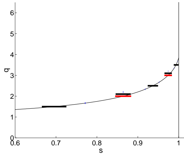
Figure 4.14: q profile for shot 70475 together with islands symbolized by horizontal bars, the widths of which were calculated as explained in chapter 3. Here are represented the islands generated by the n = 1 (lower, red bars), n = 2 (middle, black bars) and n = 3 (upper, blue bars) components of the RMPs spectrum produced by the EFCCs in n = 2 configuration.
