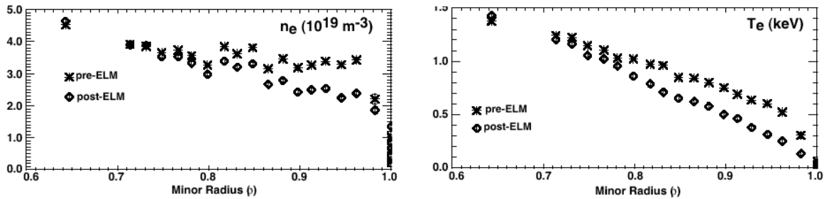
Figure 1.7: Profiles of the electron density (left) and electron temperature (right) just before and just after a type I ELM.
