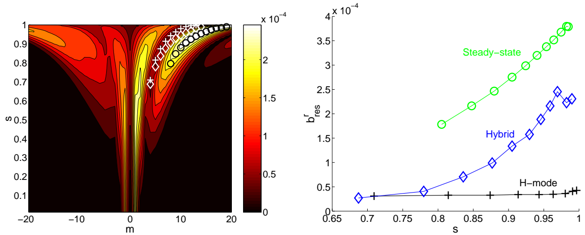
Figure 5.30: Left: spectrum of 2|\tilde{b}_{m,-3}^1| (dimensionless quantity) for the blanket coils with an optimized phasing for q_{95} = 5 , with symbols showing the resonance (white '+'s for the H-mode, blue diamonds for the hybrid-like q profile and green circles for the steady-state-like q profile). Right: corresponding profile of b_{res}^r for 20kAt in the coils (diamonds [resp. circles] correspond to a hybrid-like [resp. steady-state-like] q profile, see section 5.6).
