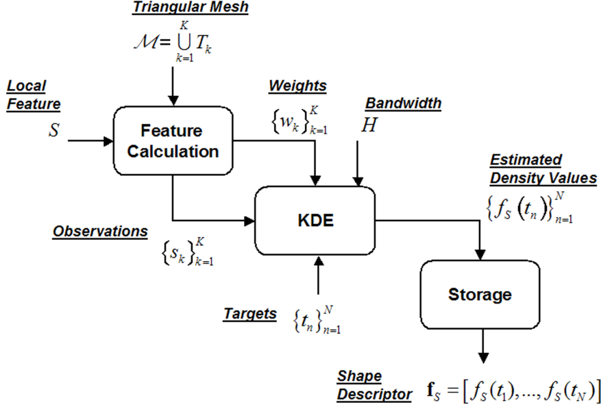
Figure 2.11: Flow diagram of density-based shape description algorithm
