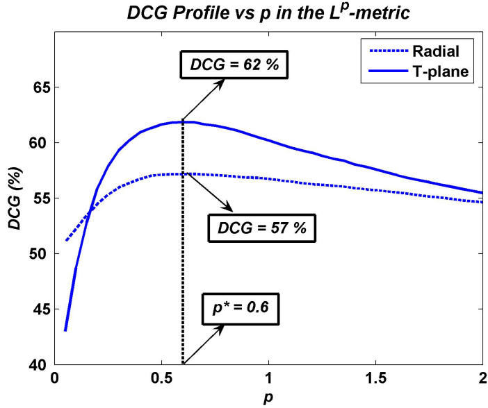
Figure 4.9: DCG Performance vs. the p parameter in the L^p -metric
