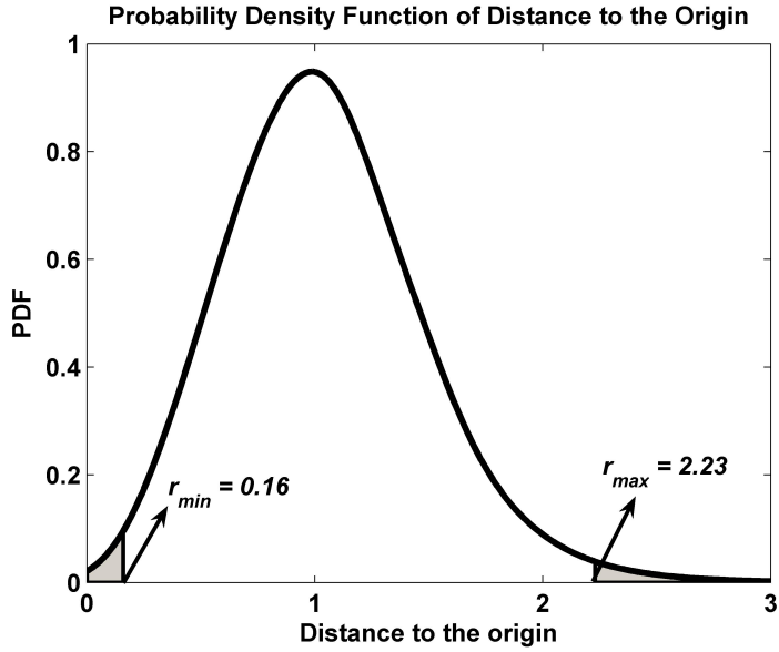
Figure 2.6: Probability density function of R displayed with the lower and upper 1% tails clipped
