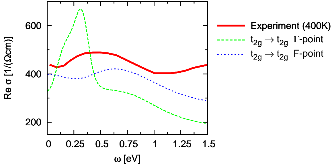
Figure 6.13 : Optical conductivity for metallic V_2O_3 . Shown is a comparison between our theoretical curve for [x0z]=[0.133 \ 0 \ 0.041] polarization with experimental results for T = 400 \text{ K} [Qazilbash(2007)]. In particular shown are two contributions to the total conductivity at different points in the Brillouin zone, as indicated. Note that here the theoretical curves were rescaled such that the total conductivity matches the experimental one at 0.5 eV.
