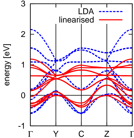
Figure 5.12 : Comparison between LDA bands and the renormalized band-structure, constructed from a linearized self-energy, according to Section A, Chapter 3.
