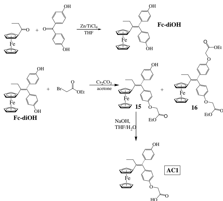
Figure 2-23: Synthetic pathway to AC1
