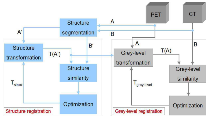
Fig. 1. General scheme of the proposed approach. Left part corresponds to the structure registration stage and the right part to the grey-level registration stage. Transformation obtained between the segmented structures initializes the registration phase that works with the whole set of intensities.
