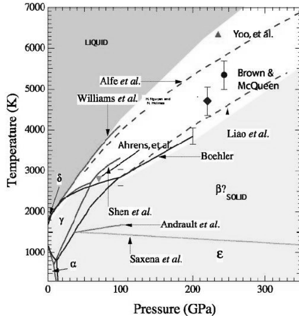
Figure 1.4: Phase diagram of Iron.
