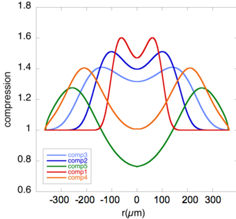
Figure 4.20: Compression values obtained from different profiles along the shock front.
