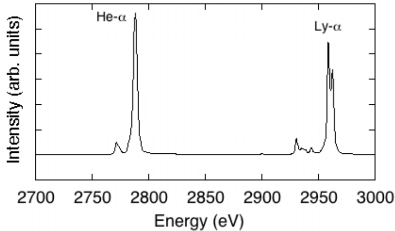
Figure 6.23: Typical emission spectrum from the Saran backlighter featuring the Ly \alpha feature at 2.96 keV with electronic satellites on lower energies. He \alpha emission is also visible at 2.79 keV with the intercombination line.
