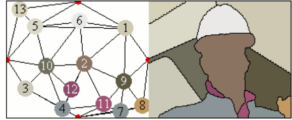
(b2) Graphe B - Partition B
