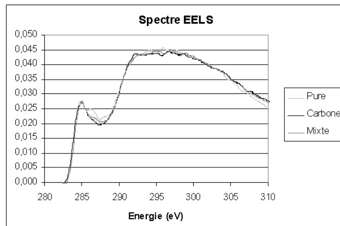
FIG. 12.1 – Spectres EELS
