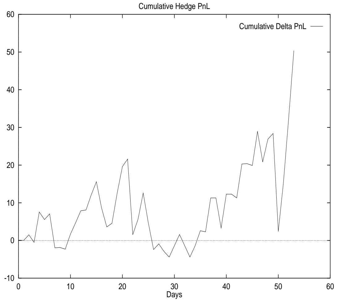
Figure 3.11: Cumulative hedging PnL generated during the trade period. This positive PnL will be offset by the option premiums and payoffs.
