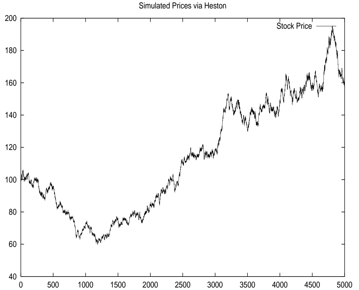
Figure 2.33: Simulated Stock-Price path via Heston using \Psi^* . This is an artificial time-series following the Heston model.
