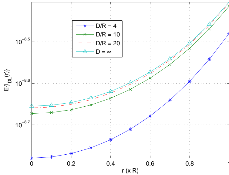
Figure 3.9: Comparison of expected downlink interference of finite network radius to an asymptotic network size. With D/R of the order 10-20, the expected downlink interference approaches the asymptotic interference.
