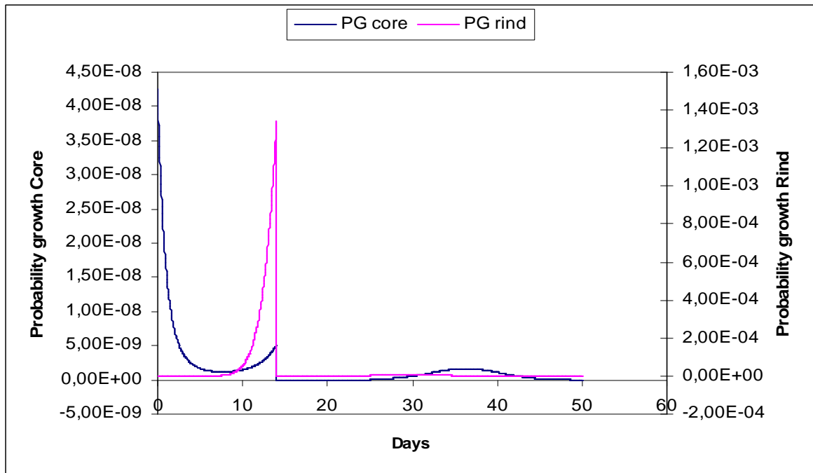
Figure 1.6 Probability of Salmonella growth in Camembert Rind and Core as predicated by the logistic regression model (in days from third day of chesse making until consumption)
