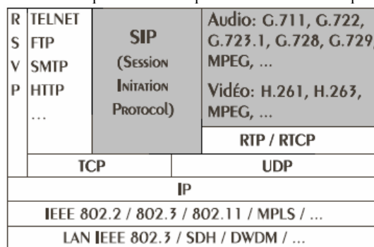
Figure 1.14 Architecture des protocoles selon SIP
