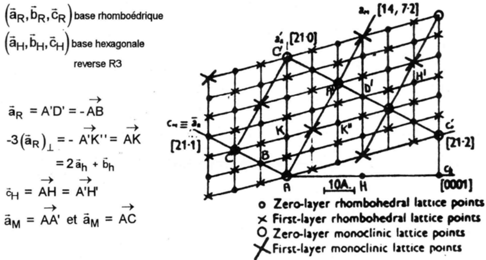
Fig. 15. The relationship between the rhombohedral and monoclinic crystal lattices. c_R is the c axis when the rhombohedral lattice is referred to hexagonal axes. a_R and c_R are the crystal axes, defining an all-face-centred lattice, corresponding to the body-centred orientation of the rhombohedral reciprocal lattice given in Fig. 14. d_R is the negative direction of one of the crystal axes of the primitive rhombohedral cell. a_M and c_M are the monoclinic crystal axes. The co-ordinate directions refer to the hexagonal axes.
