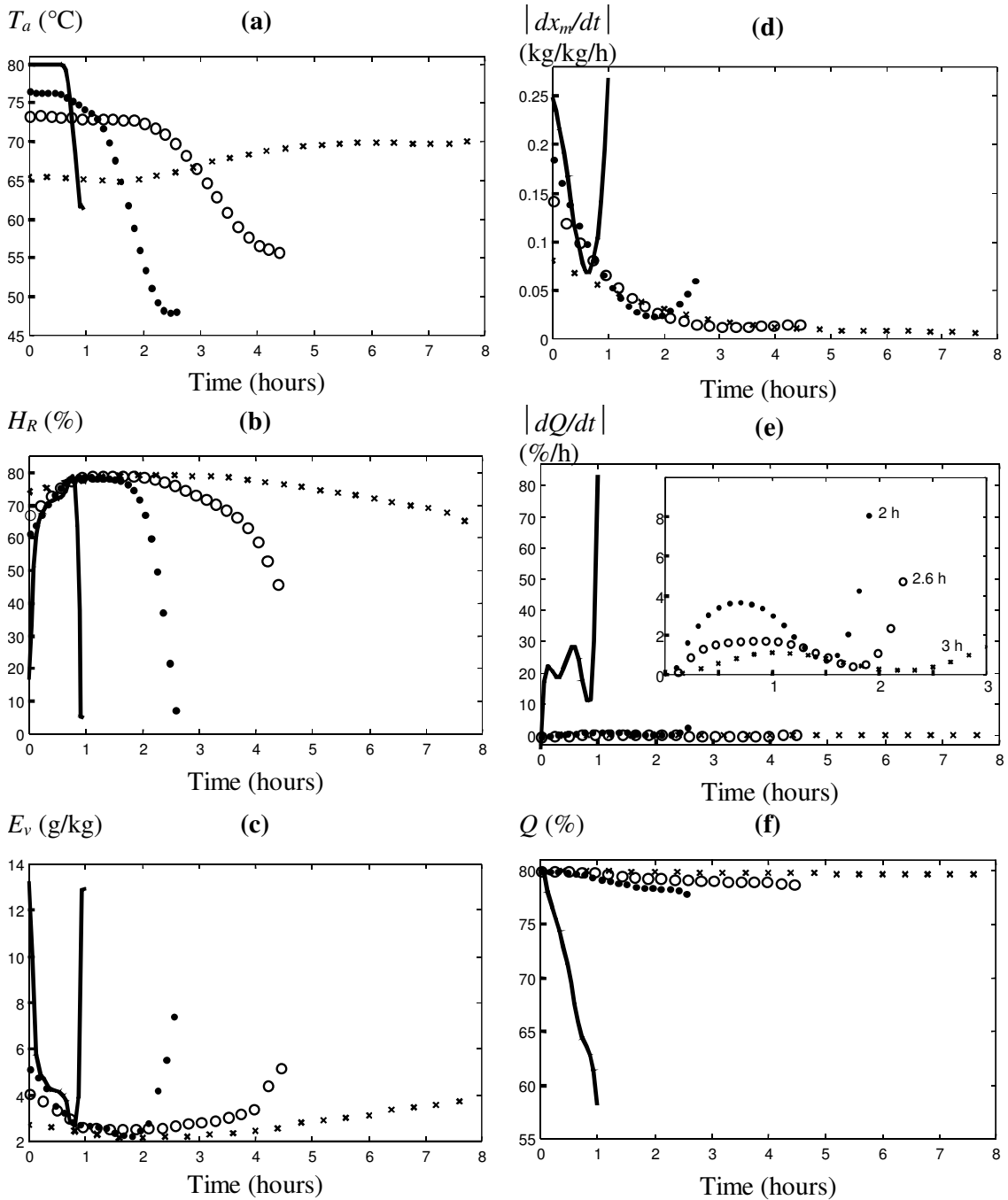
Figure 3.10. Optimal control policies for various total drying times. Symbols: (—) 1 hour, (●) 2.67 hours, (○) 4.5 hours, (x) 7.5 hours. (a) Air temperature. (b) Relative humidity. (c) Evaporation capacity of the drying air. (d) Drying rate. (e) Quality degradation rate. Insert: Quality degradation rate for short drying times. (f) Quality degradation.
