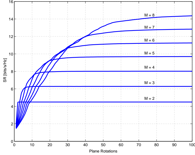
Figure 6.1: Sum rate as a function of the number of plane rotations (algorithm iterations) for different number of transmit antennas, K = M users and average SNR = 10 dB.
