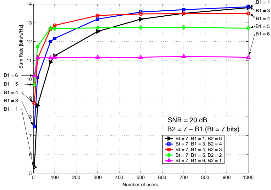
Figure 4.10: Sum rate vs. number of users for M = 2 and \text{SNR} = 20 dB.
