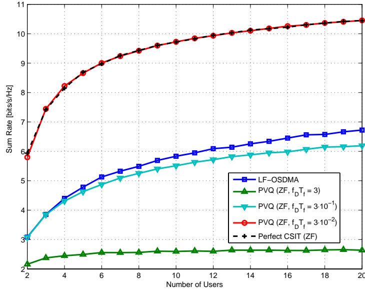
Figure 5.4: Sum rate for different number of users in a temporally correlated channel, M = 2 transmit antennas and \text{SNR} = 10 dB.
