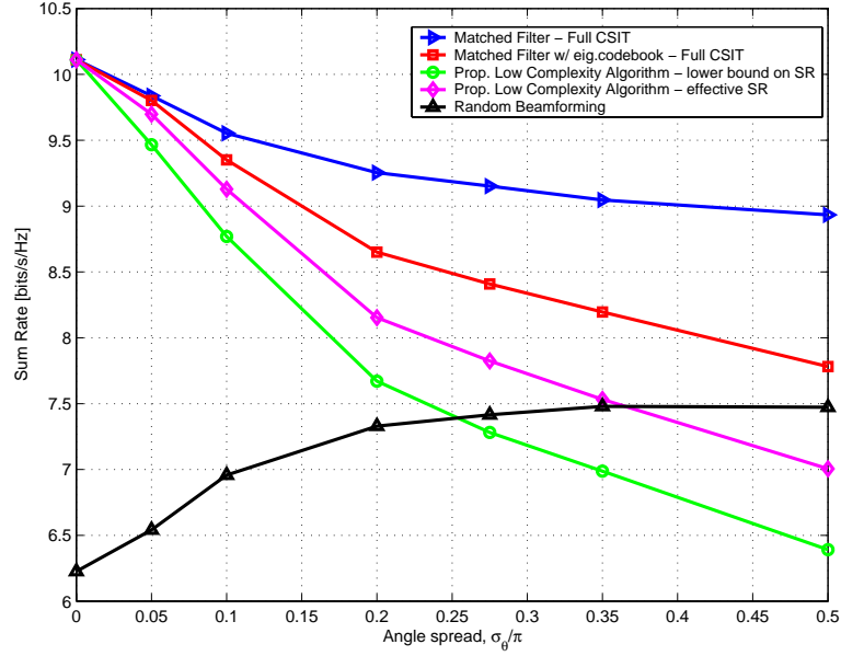
Figure 3.5: Sum rate as a function of angle spread for M = 2 transmit antennas, antenna spacing d = 0.4\lambda and K = 100 users.
