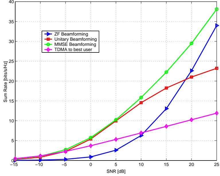
Figure 6.4: Sum rate as a function of the average SNR for M = 8 transmit antennas and K = M users.
