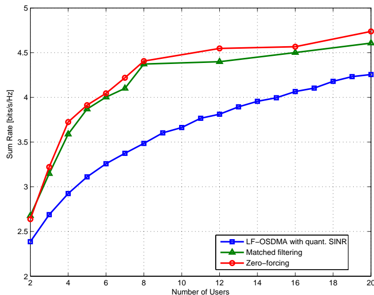
Figure 5.2: Sum rate for different number of users in a spatially correlated channel, M = 2 transmit antennas and \text{SNR} = 10 dB.
