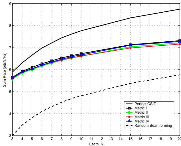
Figure 4.7: Sum rate achieved by different feedback approaches as a function of the number of users, for B = 9 bits, M = 3 transmit antennas and average SNR = 10 dB.
