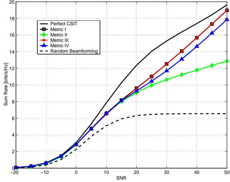
Figure 4.8: Sum rate achieved by different feedback approaches versus average SNR, for B = 9 bits, M = 3 transmit antennas and K = 10 users.
