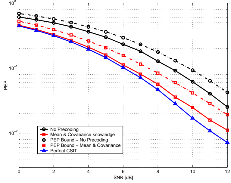
Figure 2.1: PEP vs. SNR for different CSIT levels, \rho = 0.9 and \gamma = 40\%
