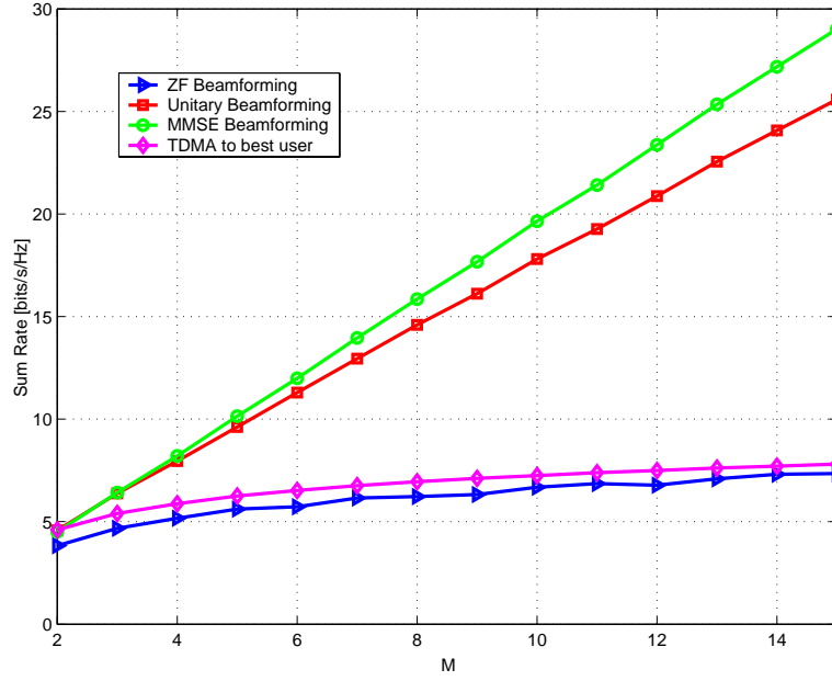
Figure 6.3: Sum rate as a function of the number of antennas M for K = M users and average SNR = 10 dB.
