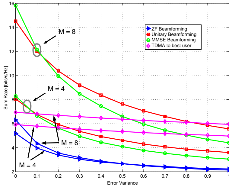
Figure 6.5: Sum rate as a function of the channel estimation error variance for M = 4, 8 transmit antennas, K = M users and average SNR = 10 dB.
