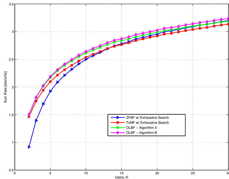
Figure 3.2: Sum rate as a function of the number of users for M = 2 transmit antennas, and average SNR = 0 dB.
