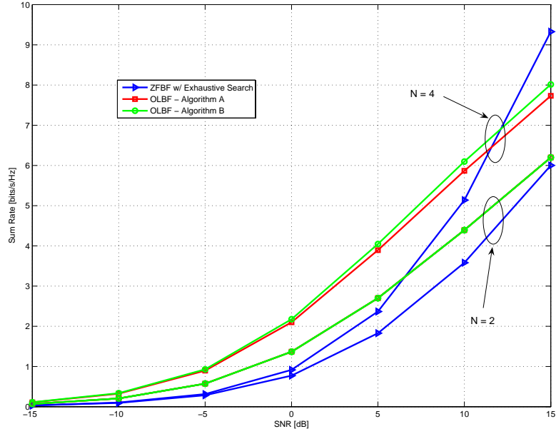
Figure 3.1: Sum rate as a function of the SNR for M = 2, 4 transmit antennas and K = M users.
