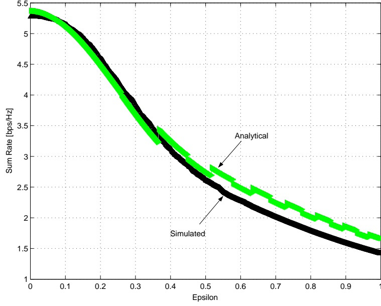
Figure 4.3: Comparison of analytical and simulated lower bounds on the sum rate using Metric III, for M = 2 antennas, K = 15 users, \text{SNR} = 10 dB and B = 1 bit.
