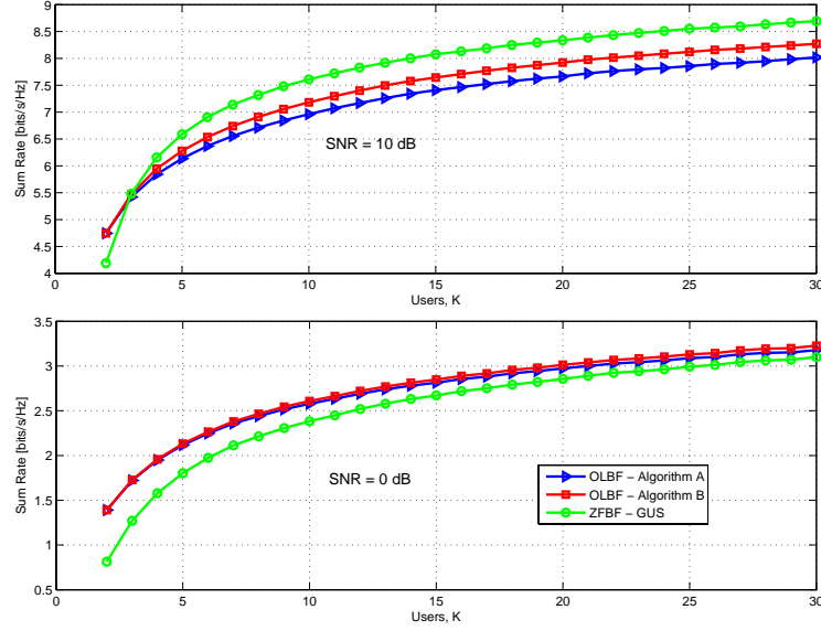
Figure 3.3: Sum rate comparison of suboptimal beamforming approaches as a function of the number of users for M = 2 transmit antennas, for a) average SNR = 0 dB (below) and b) average SNR = 10 dB (above).
