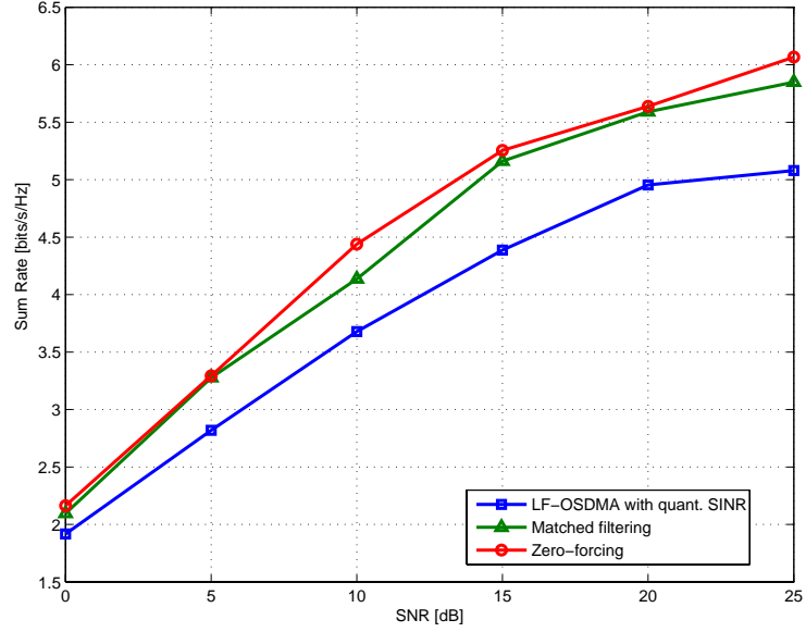
Figure 5.3: Sum rate for different SNR values in a spatially correlated channel, M = 2 transmit antennas and K = 10 users.
