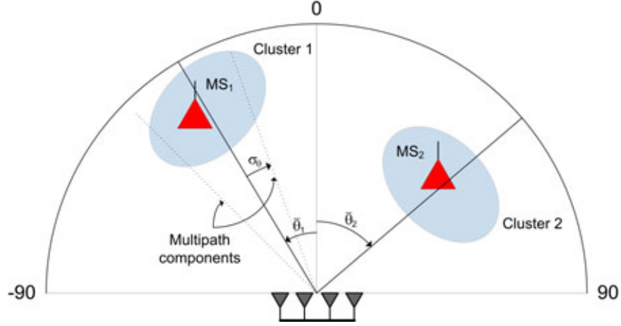
Figure 5.1: Broadcast channel model with mobile stations (MS) surrounded by local scatterers grouped in clusters, located in different mean angles of departure (AoD) with respect to uniform linear array (ULA) broadside.
