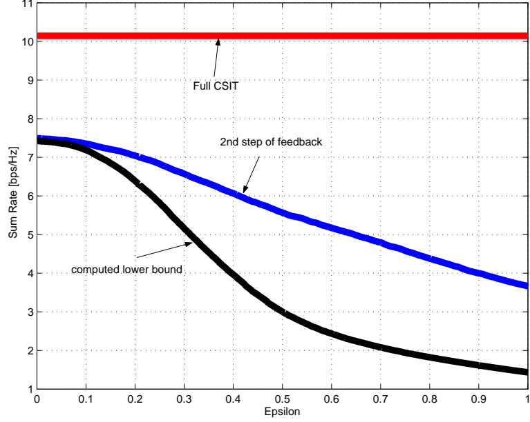
Figure 4.6: Comparison of simulated lower bound on the sum rate using Metric III, and actual sum rates obtained with second step of feedback and full CSIT. M = 2 antennas, K = 10 users, \text{SNR} = 20 dB and B = 1 bit.
