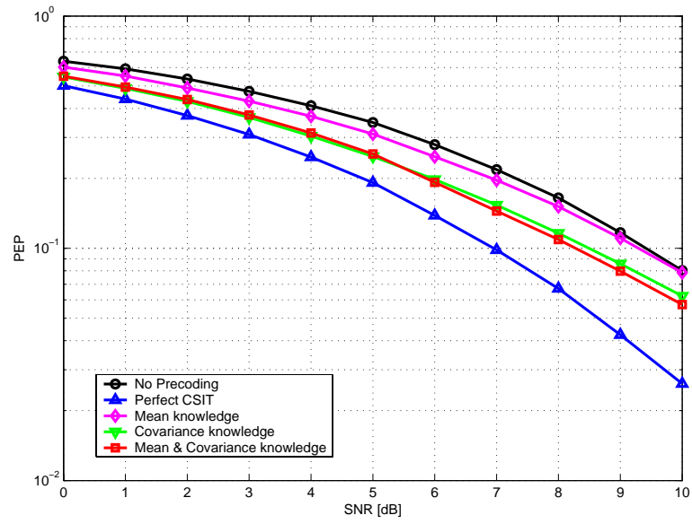
Figure 2.2: PEP vs. SNR for different CSIT levels, \rho = 0.9 and \gamma = 20\%
