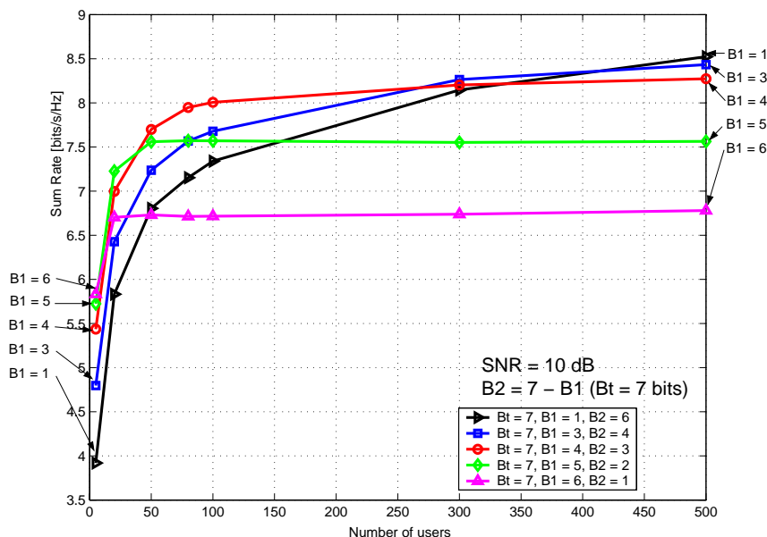
Figure 4.9: Sum rate vs. number of users for M = 2 and SNR = 10 dB.
