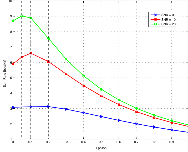
Figure 4.4: Simulated lower bound on the sum rate using Metric III as a function of the orthogonality factor \epsilon for large K .
