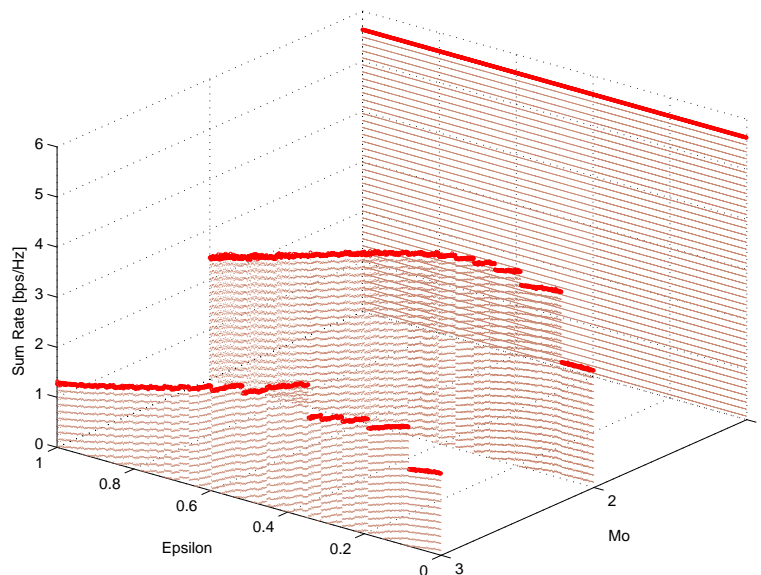
Figure 4.2: Sum-rate function using Metric I versus orthogonality factor \epsilon and number of active beams M_o , for K = 35 users, \text{SNR} = 10 dB and B = 1 bit.
