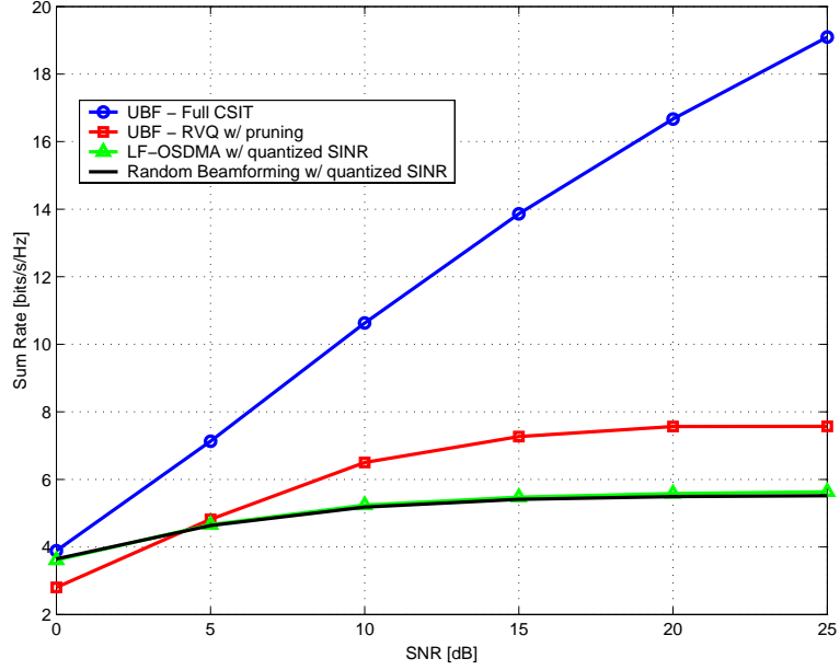
Figure 6.7: Sum rate as a function of the average SNR in a system with joint beamforming and user scheduling, M = 4 transmit antennas, K = 10 users, and B = 10 feedback bits.
