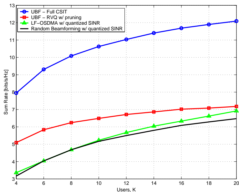
Figure 6.6: Sum rate as a function of the number of users in a system with joint beamforming and user scheduling, M = 4 transmit antennas, \text{SNR} = 10 dB, and B = 10 feedback bits.
