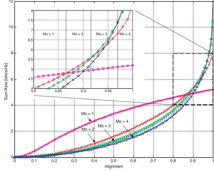
Figure 4.1: Approximated lower bound on the sum rate using Metric I versus the alignment ( \cos \theta_k ) for M = 4 antennas, variable number of active beams M_o , orthogonality factor \epsilon = 0.1 and SNR = 10 dB.
