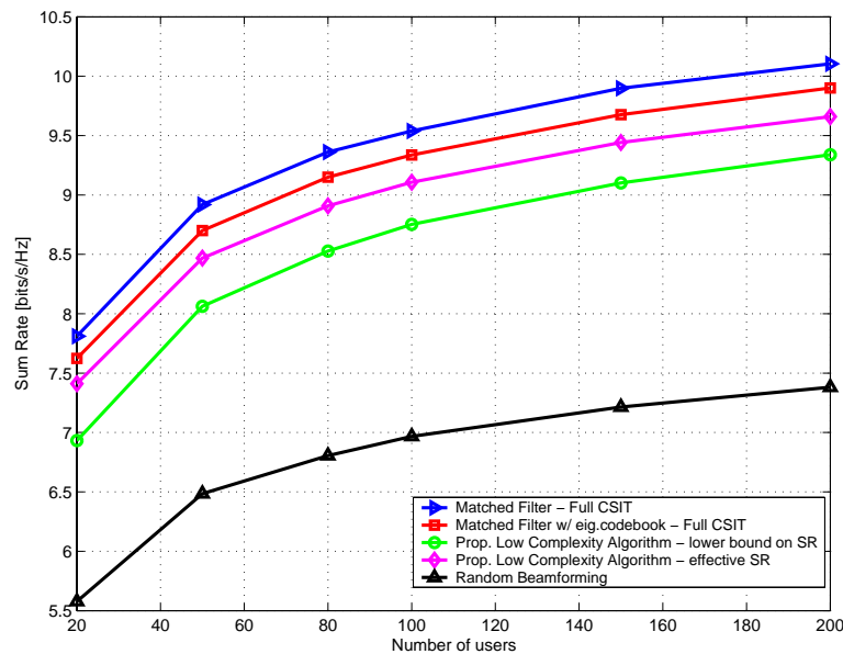
Figure 3.4: Sum rate as a function of the number of users for M = 2 transmit antennas, and \sigma_\theta = 0.1\pi .
