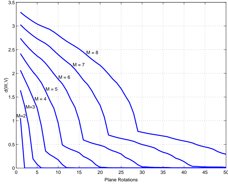
Figure 6.2: Convergence of unitary beamforming matrix for different number of transmit antennas.
