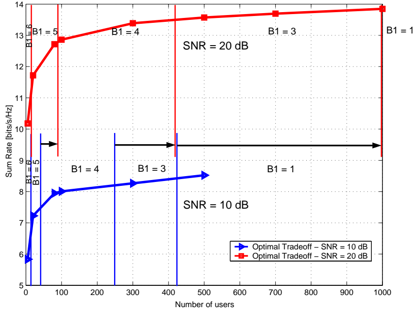
Figure 4.11: Sum rate vs. number of users in a system with optimal B_1/B_2 balancing for different SNR values.
