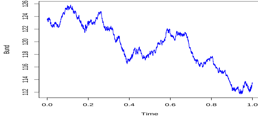
Figure I.6: The Bund contract from 2005-07-27 to 2007-08-24, sampling period of one data per hour.
