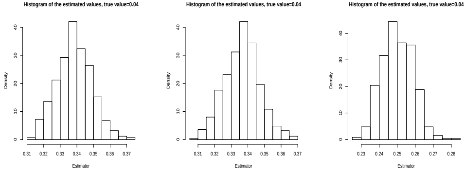
Figure II.9: Histograms of \tilde{\theta}_n(6) , \hat{\theta}_n(0.5, 5, 3) and \tilde{\theta}_n(0) for \sigma = 0.2 , n = 2^{14} and \alpha_n = 2^{-6} , 500 simulations.
