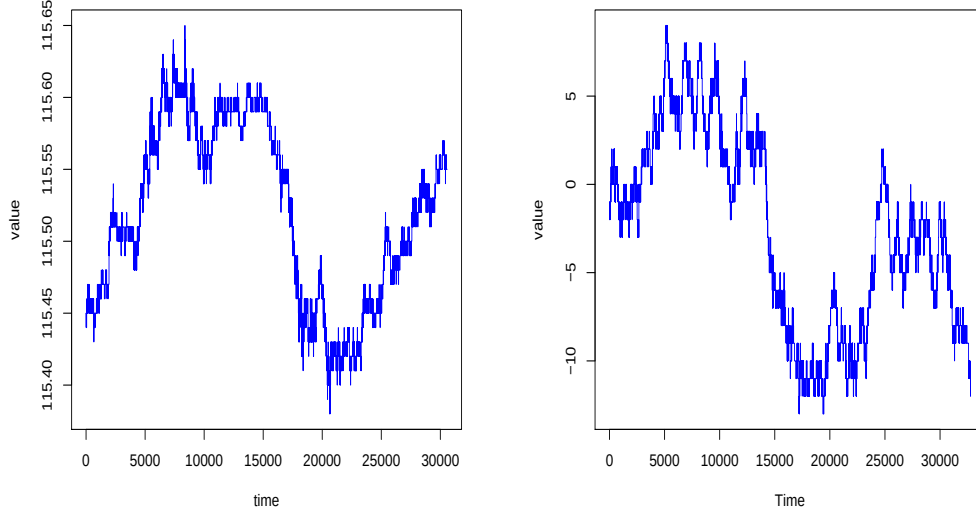
Figure II.1: Bund contract, 2007-05-06, one data every second (left), \lfloor 20W_t \rfloor , frequency = 2^{15} on [0,1] (right).
