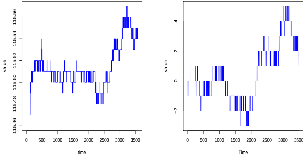
Figure II.2: Bund contract, 2007-05-06, from 10 am to 11 am, Paris time, one data every second (left), \lfloor 20W_t \rfloor , frequency = 2^{15} on [0,0.1] (right).
