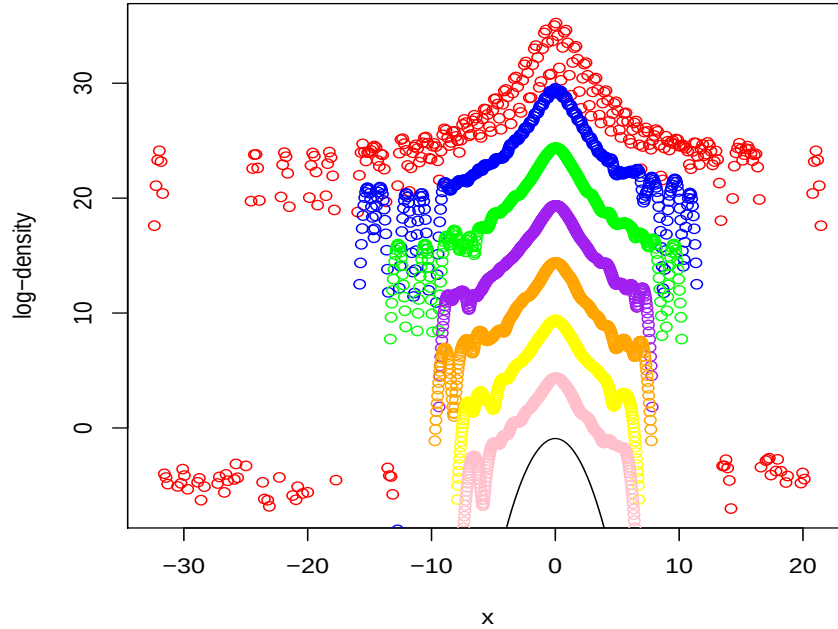
Figure E.2: Logarithms of the kernel estimations of the densities of the log return at 1 (red), 5 (blue), 10 (green), 20 (purple), 30 (orange), 45 (yellow) et 60 (pink) minutes of the Bund contract, centered and normalized, from 01/09/2005 to 31/01/2007, from 9 am to 18.30, Paris time. The log-density of a standard Gaussian variable is in colored in black. The log-density are shifted up for reading convenience. The tails are fatter than for a Gaussian variable. The smallest the sampling period, the fattest the tails.
