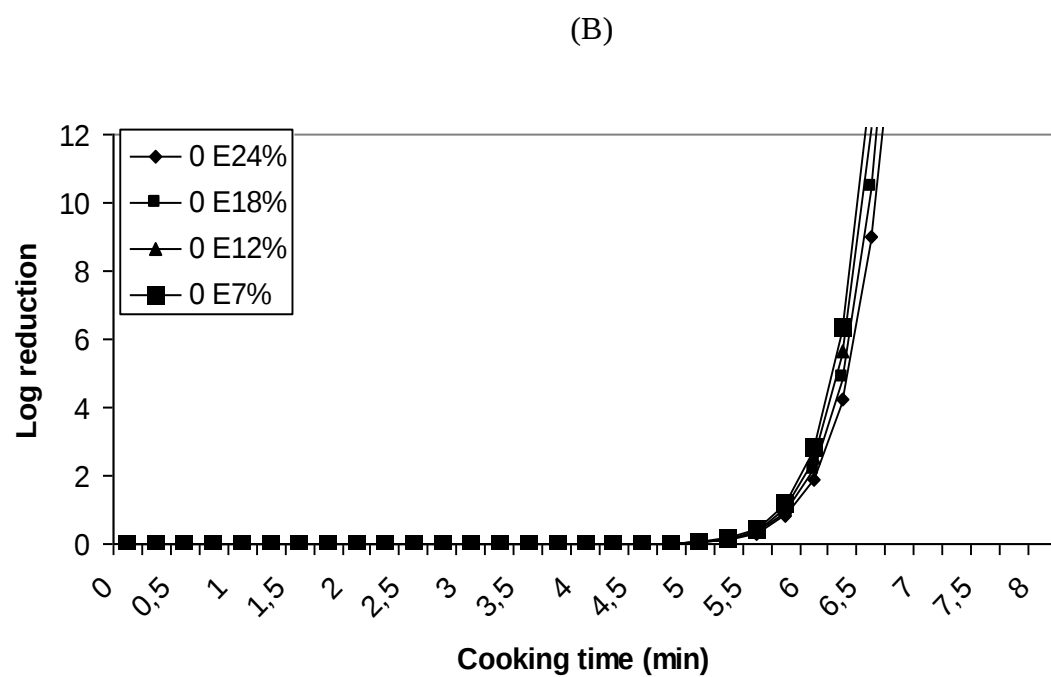
Figure 9.5. log reductions of Salmonella during time cooking at various fat content of the frozen patties ( T_{\text{initial}} = -6^{\circ}\text{C} ) (A) and the chilled patties ( T_{\text{initial}} = 4^{\circ}\text{C} ) (B) at pan temperature of 180^{\circ}\text{C} with three flippings.
