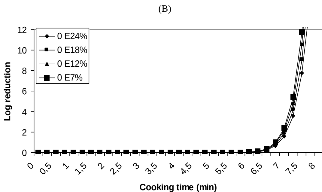
Figure 8.5. log reductions of Salmonella during time of cooking at various fat content of the frozen patties ( T_{\text{initial}} = -6^{\circ}\text{C} ) (A) and the chilled patties ( T_{\text{initial}} = 4^{\circ}\text{C} ) (B) at pan temperature of 160^{\circ}\text{C} with three flippings.
