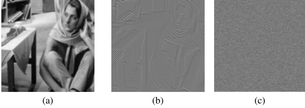
Fig. 5.4: (a) Projection of the observations set on the first eigenvector of Barbara image (b) Projection of the observation set on the 17 th eigenvector (c) Projection of the observations set on the Last eigenvector (49 th )
