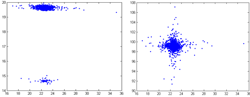
Fig. 3.3: Density plot of independent components \mathbf{s} = \mathbf{W} \cdot \Theta , independence and Gaussian mixture estimation of components appears relevant.
