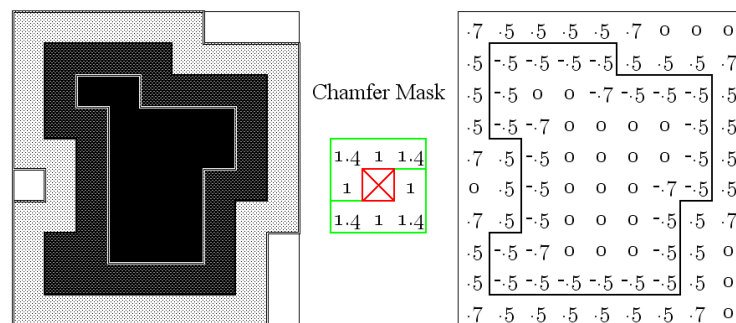
Fig. B.6: Initialisation of distance from binary images
