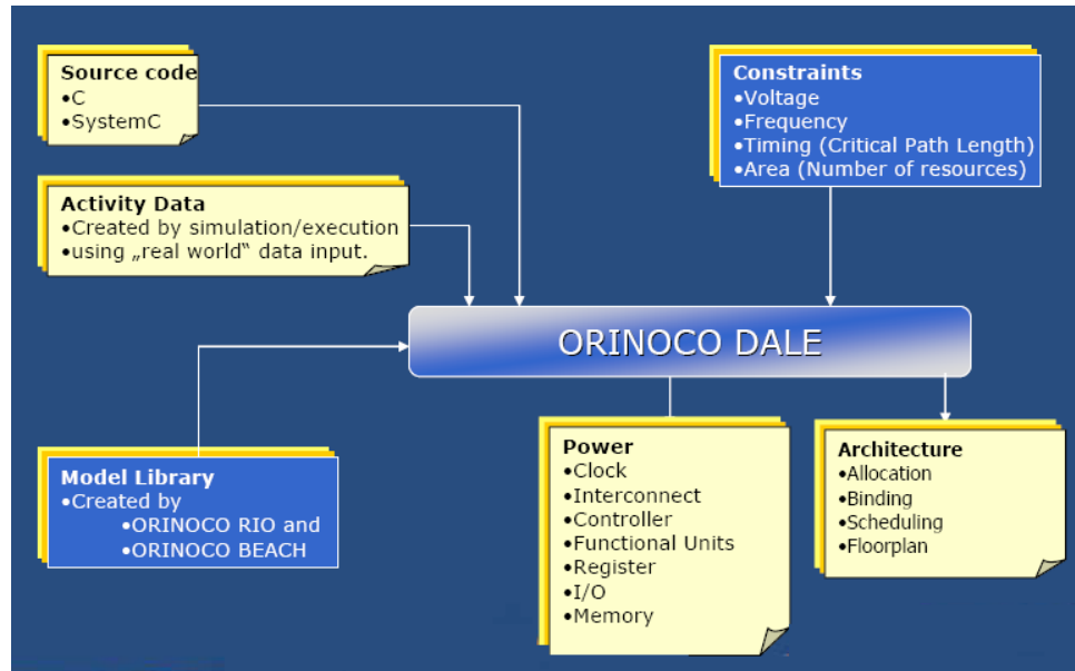
Figure 4-7 Behavioral Synthesis Flow using Orinoco Dale
