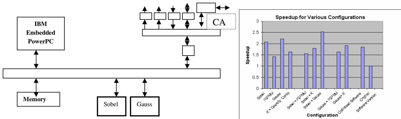
Figure 4-23 a) Platform configuration 7 (b) full HW/SW Design Space Exploration Results
