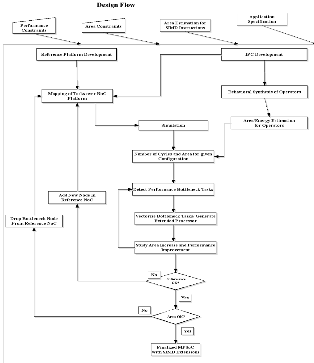
Figure 5-3 MPSoC Design Methodology for SIMD extended processor with an underlying NoC
