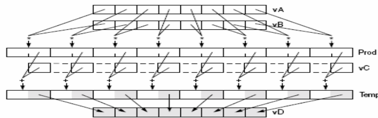
Figure 3-3 vmladduhm : Multiply-Add of Eight Integer Elements (16-Bit)
