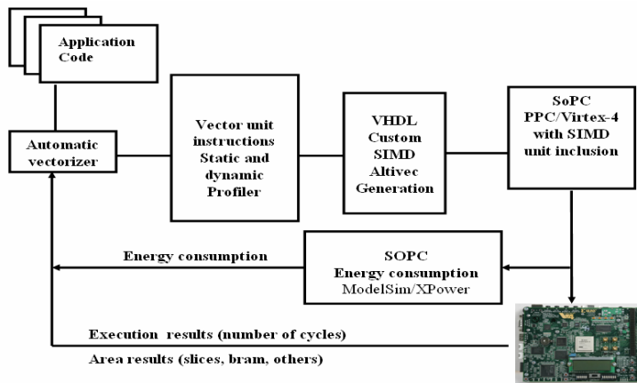
Figure 3-10 System Design Flow
