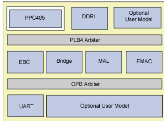
Figure 4-4 PowerPC 405 block diagram for the PEK SoC design
