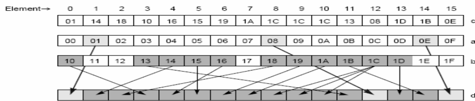
Figure 3-8 AltiVec Vector Permute Instruction
