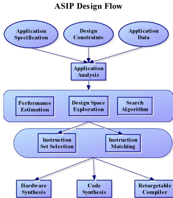
Figure 2-3 Generalized ASIP Design Flow
