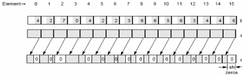
Figure 3-4 AltiVec Shift Instruction
