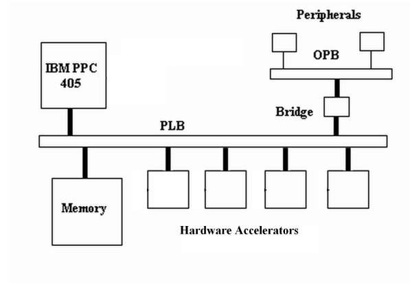
Figure 4-8 Target Platform Built using IBM TLM
