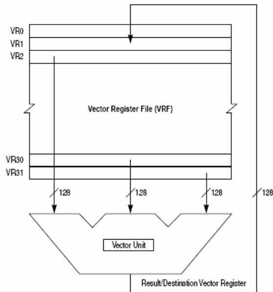
Figure 3-2 AltiVec Architecture: A System Level View
