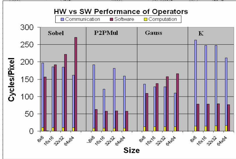
Figure 4-22 HW vs. SW Performance of Operators
