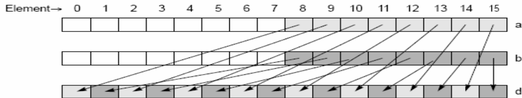
Figure 3-5 AltiVec Merge Instruction
