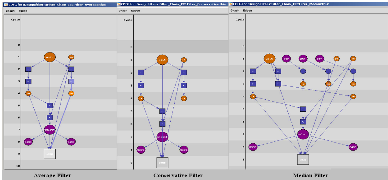
Figure 4-12 Control Data Flow Graph of Filters in the Application
