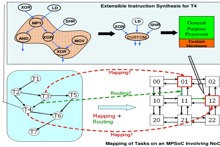
Figure 5-2 Integrating Extensible Instructions with MPSoC Synthesis using Traditional Design Flows
