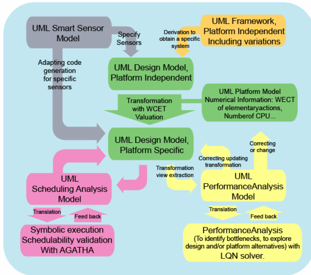
Figure 4-26 Accord/UML Design Methodology
