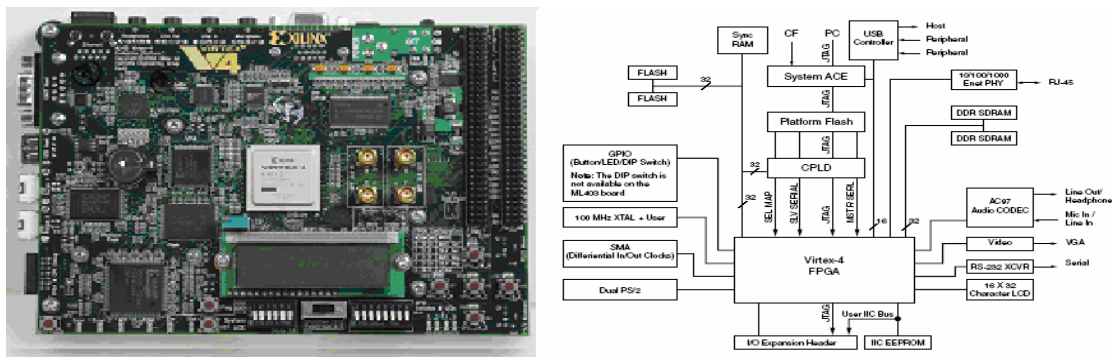
Figure 3-12 Xilinx ML403 FPGA Resources
