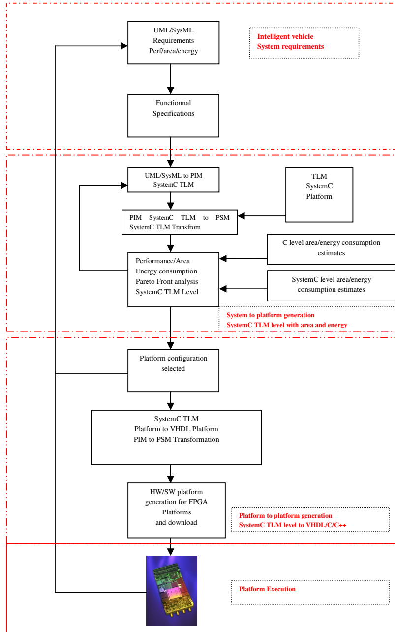
Figure 4-27 UML/SysML/TLM SystemC Platform Based design Methodology for Intelligent Vehicles
