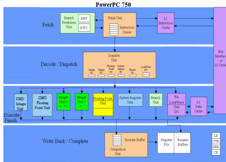
Figure 5-4 PowerPC 750 extended with AltiVec Instruction Set
