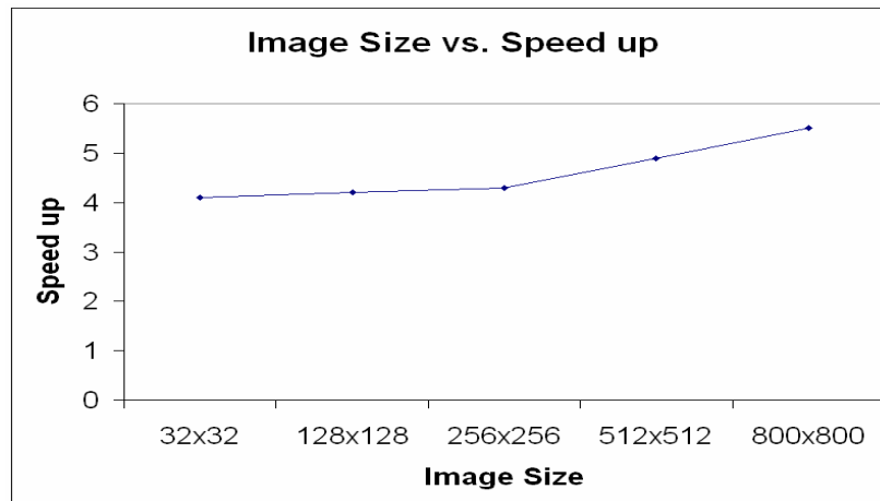
Figure 3-16 Image Size vs. Speedup Trade-off for Average Filters
