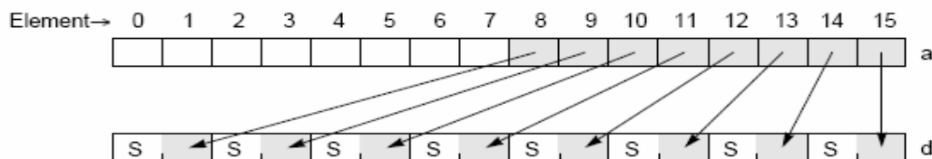
Figure 3-7 AltiVec Unpack Instruction
