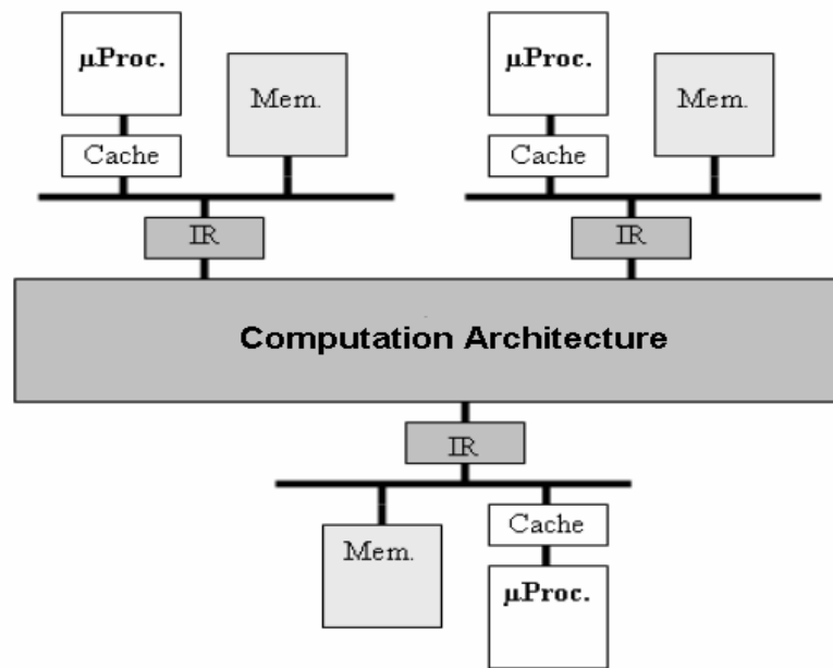
Figure 2-4 A Sample MPSoC Architecture
