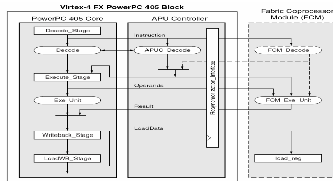
Figure 3-11 PowerPC with APU Interface
