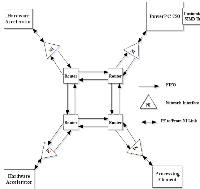
Figure 5-5 A typical Network on Chip modelled using our framework
