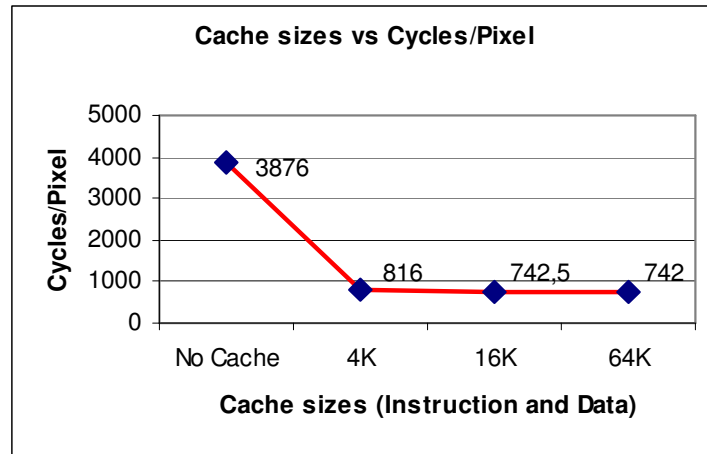
Figure 4-24 Various Cache Sizes and System Performance
