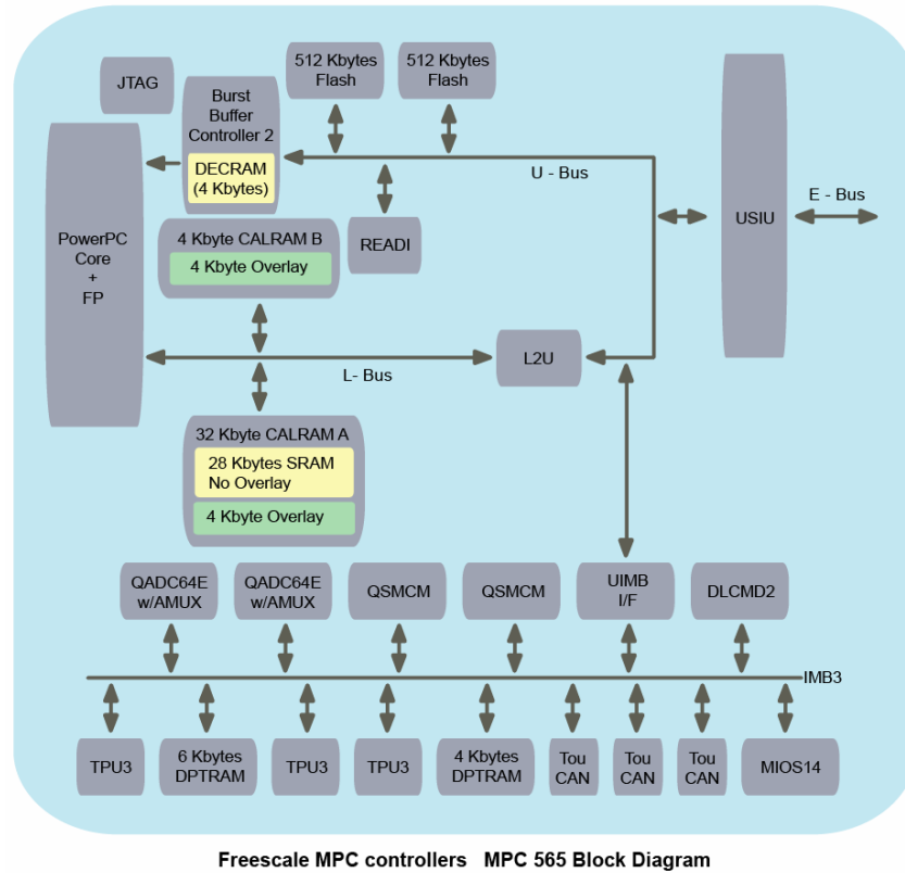
Figure 4-19 Freescale MPC controllers (b) MPC 565 Block Diagram
