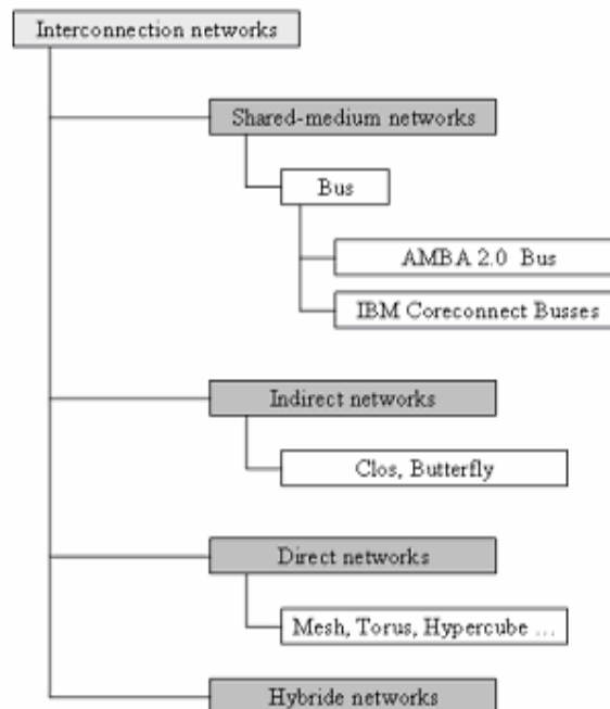
Figure 2-5 Classification of Communication Architectures
