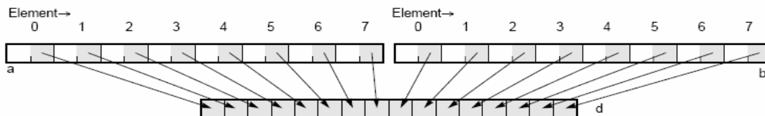
Figure 3-6 AltiVec Pack Instruction
