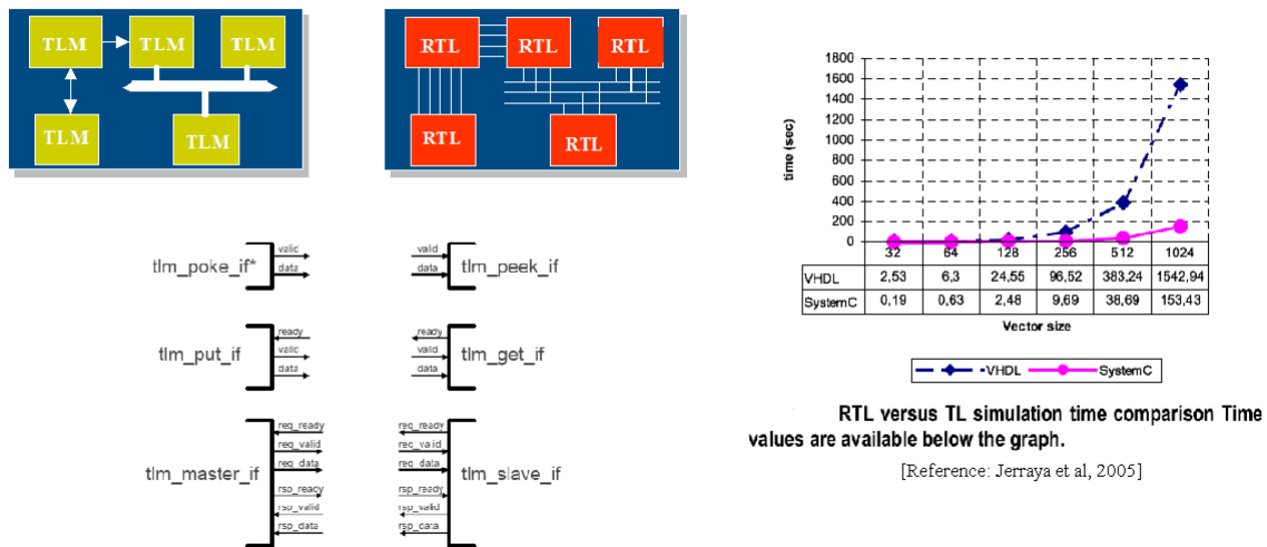
Figure 4-1 Transaction Level Modeling vs. Register Transfer Level
