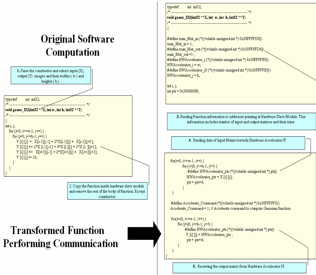
Figure 4-11 Transforming SW Computation into Communication Tasks
