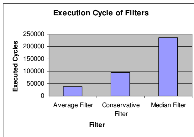
Figure 4-15 Execution cycles taken by Filters
