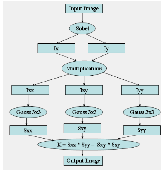
Figure 4-17 Harris Corner Detector Chain
