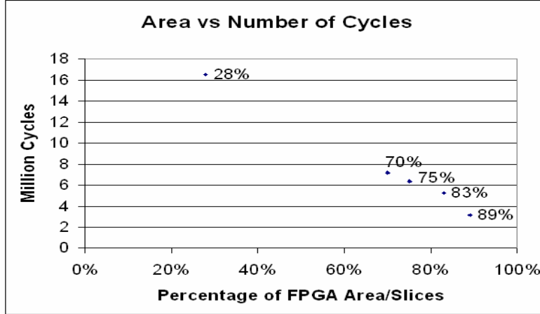
Figure 3-14 Area vs. Speedup Trade-off for Matrix Transpose Program
