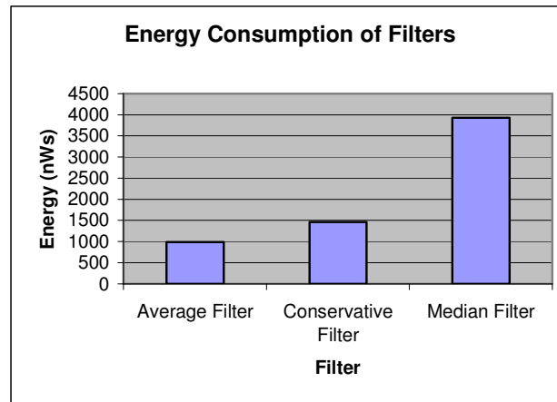
Figure 4-13 Energy consumption requirements for filters
