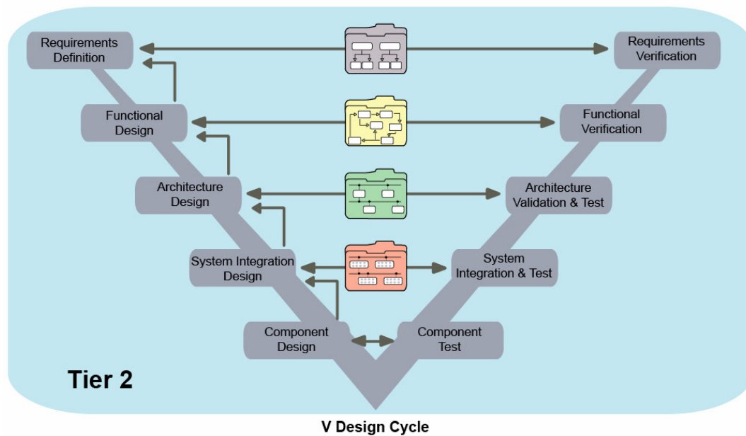
Figure 4-20 V Design Cycle
