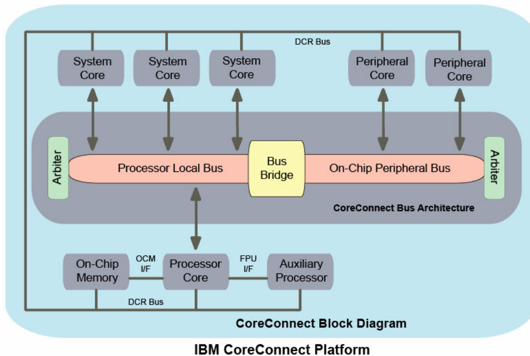
Figure 4-2 IBM CoreConnect Platform
