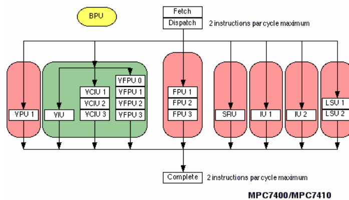
Figure 3-1 PowerPC G4 Architecture
