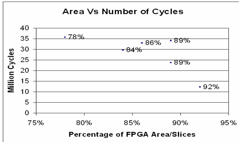
Figure 3-15 Area vs. Speedup Trade-off for Average Filters
