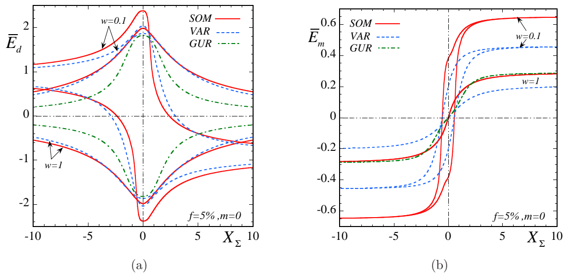
Figure 4.15: Macroscopic strain-rates obtained by the SOM as a function of the porosity f and the stress triaxiality X_\Sigma for two values of the aspect ratio w = 1, 0.1 . (a) shows the deviatoric part \bar{E}_{11} - \bar{E}_{22} and (b) shows the hydrostatic part \bar{E}_m of the macroscopic strain-rate for an ideally-plastic matrix phase m = 0 . VAR and GUR estimates are shown for comparison.
