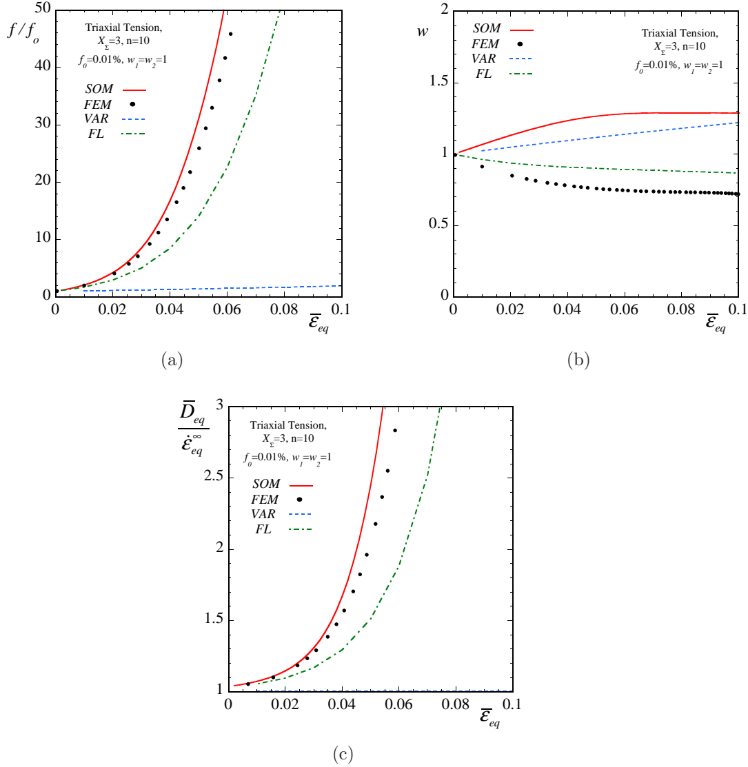
Figure 7.18: Results are shown for the evolution of the relevant microstructural and macroscopic variables for a porous material consisted of initially spherical pores embedded in a matrix with exponent n = 10 as a function of the axial macroscopic strain \bar{\epsilon}_{eq} . The initial porosity is f_o = 0.01\% and the material is subjected to axisymmetric triaxial tension loading ( X_\Sigma = 3 and T/S = 0.727 with S/|S| > 0 ) so that the voids evolve into prolate spheroids with aspect ratio w_1 = w_2 = w > 1 . The SOM and the VAR estimates are compared with FEM results and the recent Flandi-Leblond (2005) model ( FL ) for the evolution of the (a) porosity f , (b) the aspect ratio w and (c) the normalized axial strain-rate \bar{D}_{eq}/\dot{\epsilon}_{eq}^\infty ( \dot{\epsilon}_{eq}^\infty is the corresponding strain-rate in the absence of voids).
