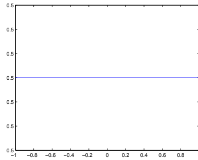
FIG. 6.22 – \theta^+ at t = 0 .
