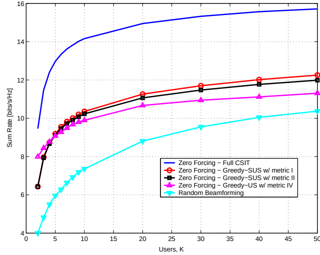
Figure 5.3: Sum rate as a function of the number of users for B_D = 4 bits, M = 2 transmit antennas and \text{SNR} = 20 dB.
