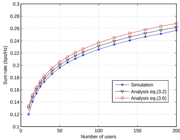
Figure 3.3: Achievable sum rate comparison between simulated and analytical results for RBF with M = 4 antennas and SNR = -15 dB.
