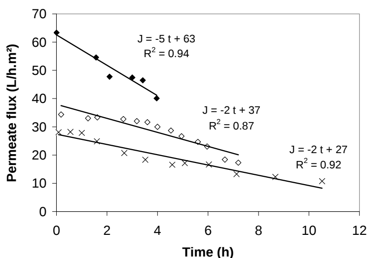
Figure 2 Time-decrease of permeate flux during microfiltration. ♦: CF1 (5 m/s, 0.26 MPa); x: CF4 (1.5 m/s, 0.26 MPa); ◇: CF8 (2.01 m/s, 0.15 MPa).
