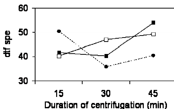
Figure 1 Interaction between centrifugation speed and duration on the loss of specific acidification activity during freezing ( dtf_{spe} , in min/log(CFU/ml)) of Lb. bulgaricus CFL1 cells. (□): 3,000g; (■):10,000g; (●): 17,000g.
