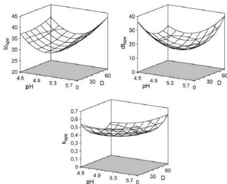
Fig. 2. Estimated response surfaces representing the effects of pH and duration ( D , in min) of acidification, on the initial specific acidification activity ( tc_{spe} , in min ( \log(\text{CFU ml}^{-1}) ) ^{-1} ), and on the loss of specific acidification activity during freezing ( dt_{spe} , in min ( \log(\text{CFU ml}^{-1}) ) ^{-1} ) and frozen storage ( k_{spe} , in min ( \log(\text{CFU ml}^{-1}) ) ^{-1} \text{ d}^{-1} ) of L. bulgaricus CFL1.
