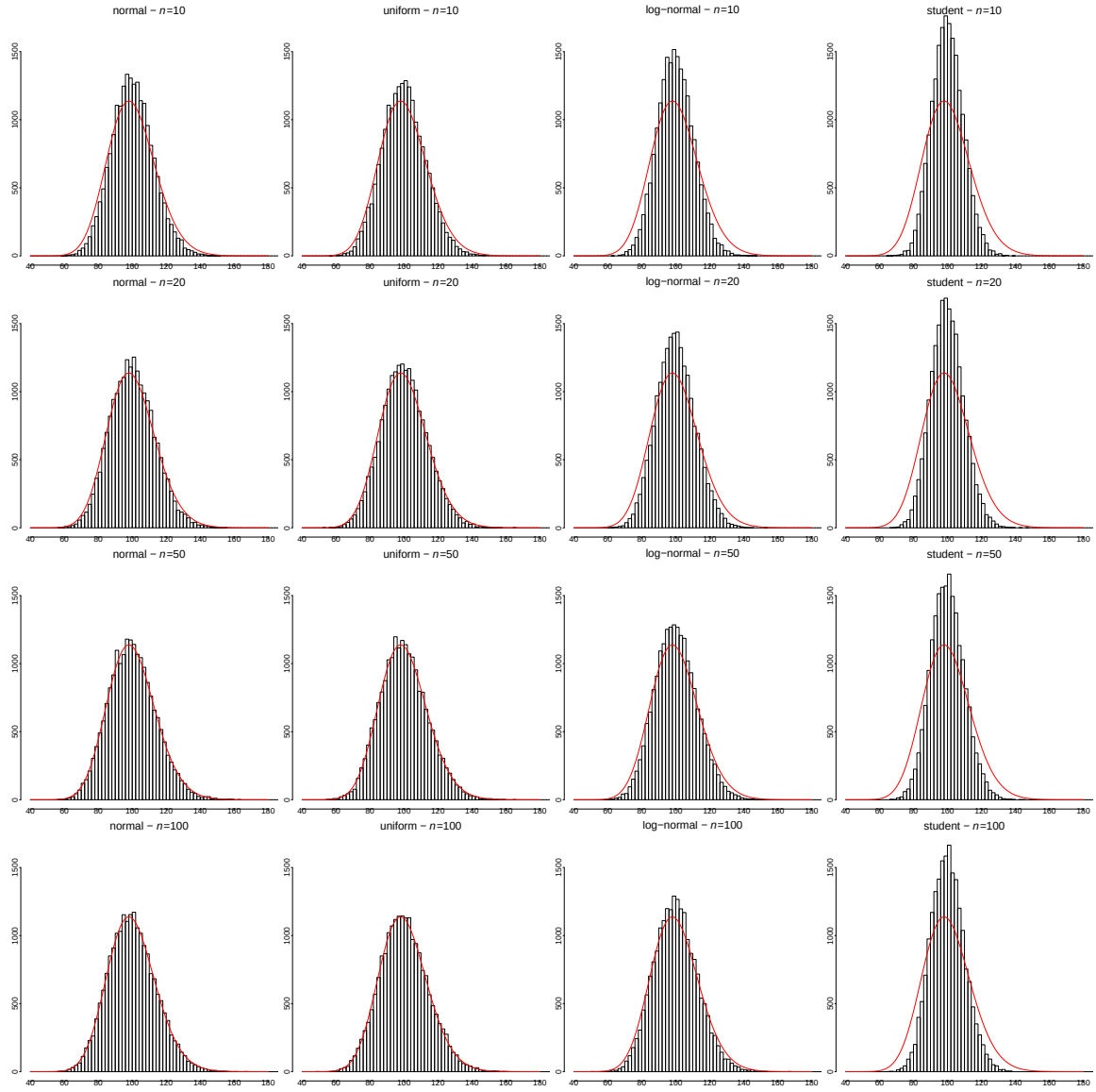
Figure A.1: Histograms for simulations under \mathbf{H}_0 without correlation - Histograms of the statistical criterion over 20000 simulations. The data have been simulated using the normal, uniform, log-normal and student distributions. n corresponds to the number of observations. The number of variables has been set at 100. The \chi^2(100) probability density function is displayed as a red line.
