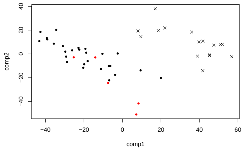
Figure 3.7: PLS components for Stransky et al. (2006) - \bullet represents patients with T2-T4 tumour (32) and \times represents patients with Ta tumour (16). The patients are represented in the first two components of the PLS. Patients with an amplification of 8q22-23 are shown in red.
