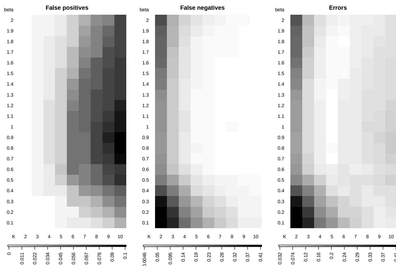
Figure 10 Comparison between qualitative assessment and segmentation results with various ( K , \beta ) – bladder cancer data set. The segmentation algorithm is run with K \in \{2, \dots, 10\} ( x axis) and \beta \in \{0.1, 0.2, \dots, 2.0\} ( y axis) and compared with the expert assessment of the breast cancer data set. (a) False positive rate; (b) False negative rate; (c) Total error rate.
