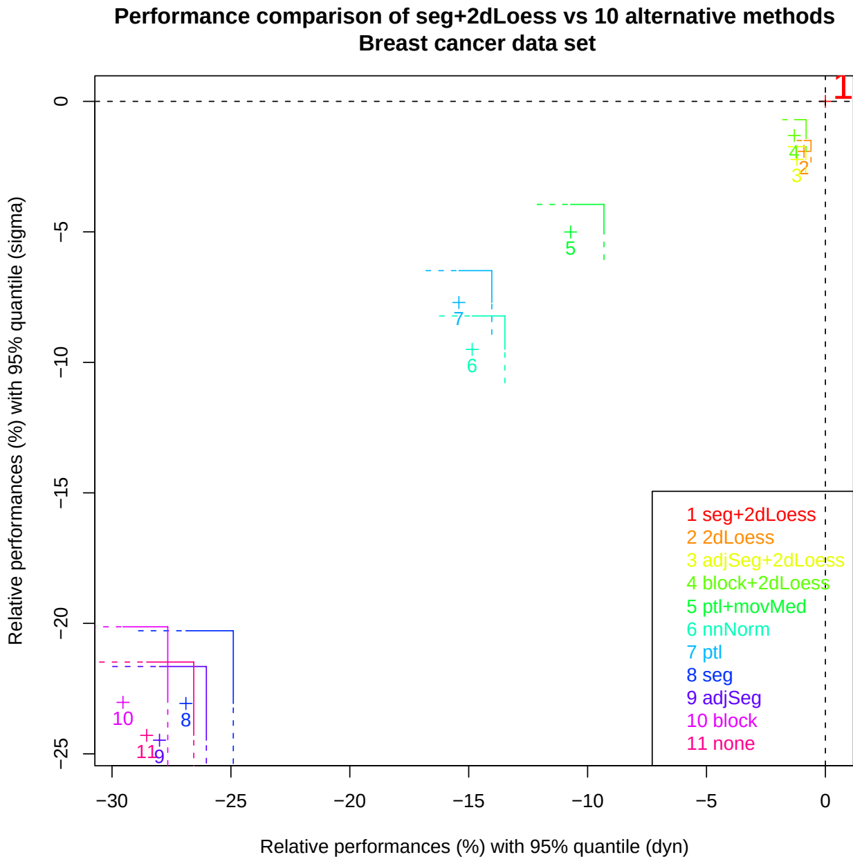
Figure 7 The proposed method (seg+2dLoess) compares favorably to all other normalization methods – breast cancer data set. We compared the proposed method (seg+2dLoess) to ten methods for two quality criteria: sigma and dyn . Each color corresponds to the comparison of seg+2dLoess with a different method. The proposed method is taken as a reference (red point 1 at (0, 0)). For each method i , the cross indicates the mean relative performance (see methods section) of the data set for dyn (x axis) and in sigma (y axis), and the lines give the corresponding 95% quantile of relative performance. For sigma ( dyn , respectively), the methods with a 95% quantile below (left to, respectively) the horizontal (vertical, respectively) dashed black line are significantly outperformed by our proposed method. Here seg+2dLoess significantly outperforms all methods for dyn and sigma .
