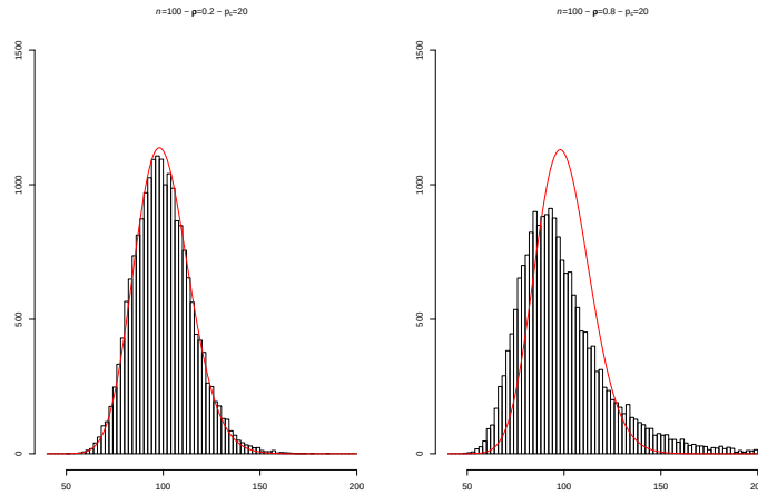
Figure 3.10: Typical histograms for simulations under \mathbf{H}_0 with correlation - Two typical histograms of the statistical criterion over 20000 simulations. The data have been simulated using the normal distribution. n corresponds to the number of observations, \rho is the correlation value, and p_c is the number of correlated variables. The number of variables has been set at 100. The \chi^2(100) probability density function is displayed as a red line.
