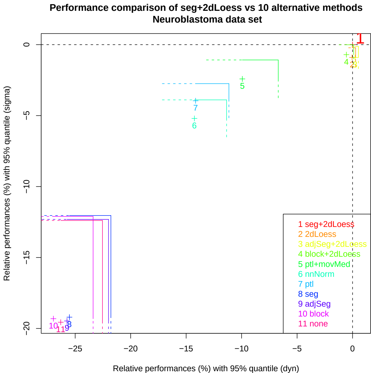
Figure 8 The proposed method (seg+2dLoess) compares favorably to all other normalization methods – neuroblastoma data set. We compared the proposed method (seg+2dLoess) to ten methods for two quality criteria: sigma and dyn . Each color corresponds to the comparison of seg+2dLoess with a different method. The proposed method is taken as a reference (red point 1 at (0,0)). For each method i , the cross indicates the mean relative performance (see methods section) of the data set for dyn (x axis) and in sigma (y axis), and the lines give the corresponding 95% quantile of relative performance. For sigma ( dyn , respectively), the methods with a 95% quantile below (left to, respectively) the horizontal (vertical, respectively) dashed black line are significantly outperformed by our proposed method. Here seg+2dLoess significantly outperforms all methods for dyn and sigma , except those containing a gradient subtraction step with 2dLoess.
