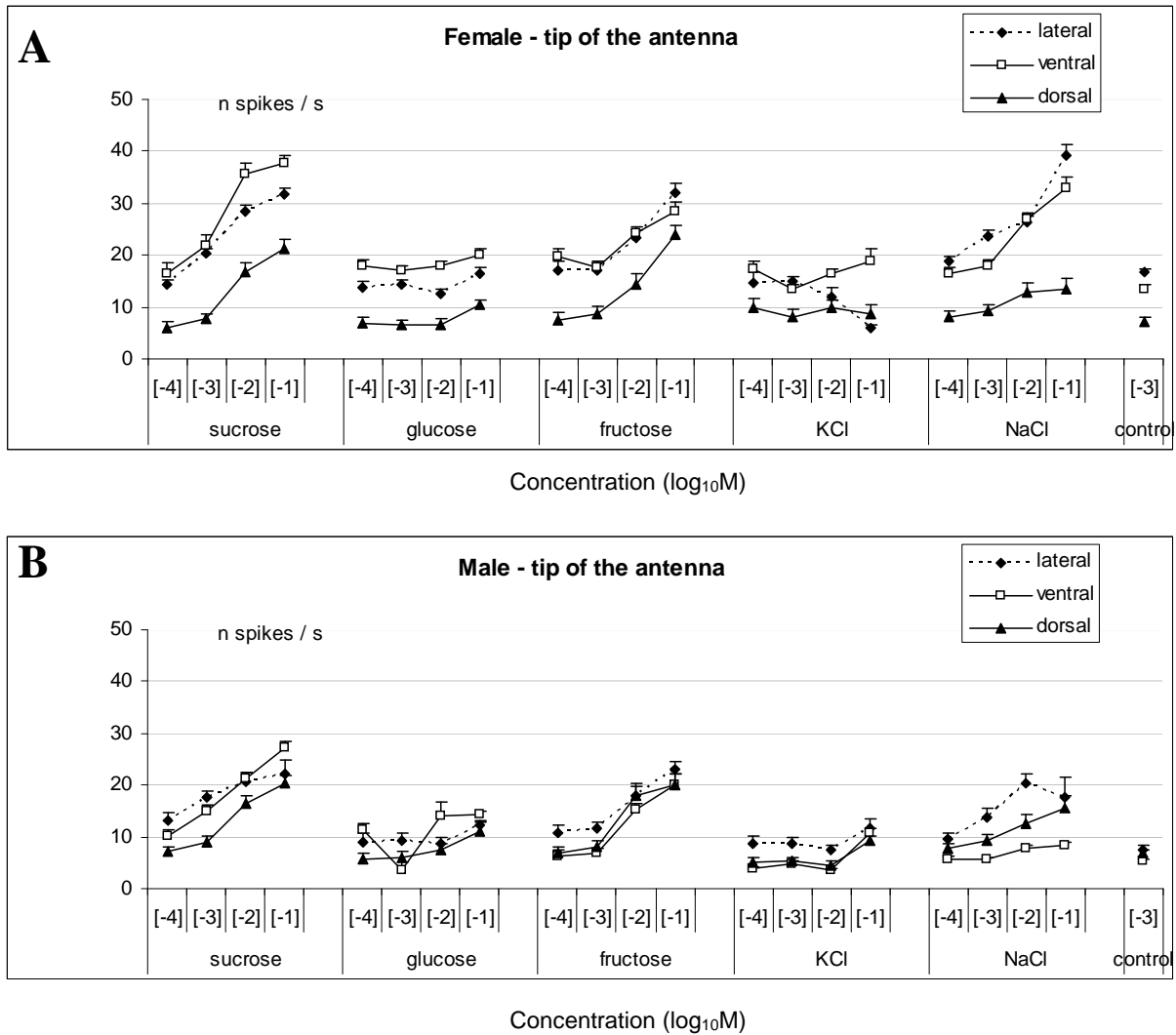
Figure 7. Dose-response curves from lateral, ventral and dorsal sensilla in response to sucrose, fructose, glucose, KCl and NaCl. A. In females (N sucrose= 25-70, N fructose = 20-40, N glucose = 35-65, N KCl= 20-40, N NaCl = 50-80, N control = 80-100). B. In males (N sucrose= 20-45, N fructose = 20-35, N glucose = 6-20, N KCl= 25-30, N NaCl = 40-85, N control = 20-70). Error bar indicates the standard error.
