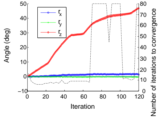
Figure 6.31: Rotation estimate without a robust function
