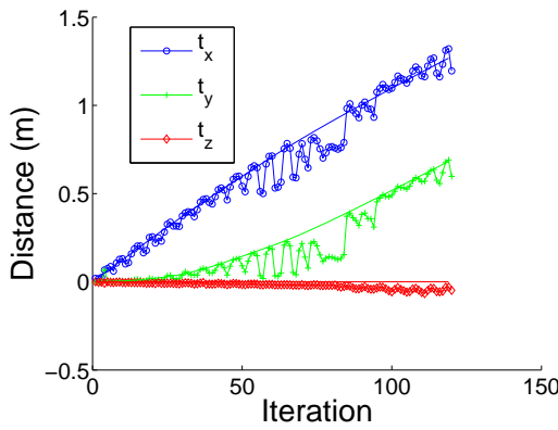
Figure 6.30: Translation estimate without a robust function
