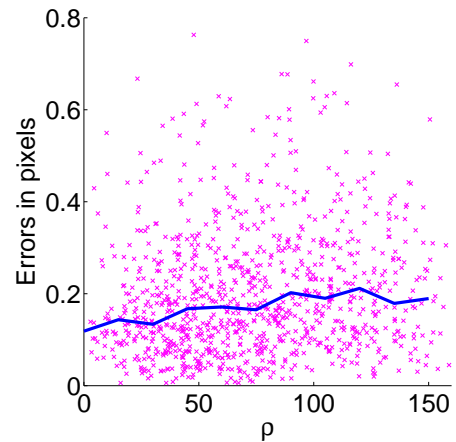
Figure 3.9: Pixel error versus distance - wide-angle sensor
