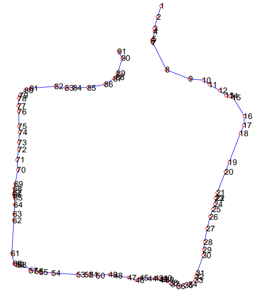
Figure 9.38: Topological map before loop closing
