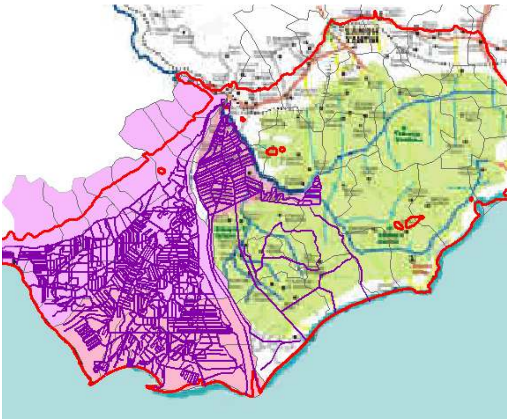
Figure 91 - Present irrigation system in the Nestos delta (in pink-magenta) and future extension to the Xanthi plain (in green-blue) in liaison with the Temenos dam project
