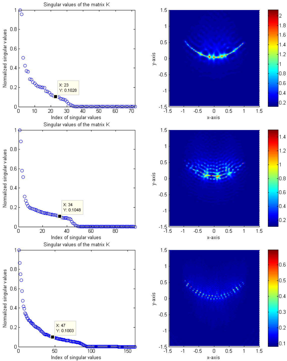
FIG. 2.11 – The distribution of normalized singular values of the matrix K (Left column) and maps of W_a(z) when a = 1 (right column), for all points z \in \tilde{\Omega} for N = 72 incidences and a 0.3 wave length (top row), for N = 96 incidences and a 0.2 wave length (center row) and for N = 160 incidences and a 0.1 wave length (bottom row) when the thin inclusion is \Gamma_5 , with dielectric contrast of 5 .
