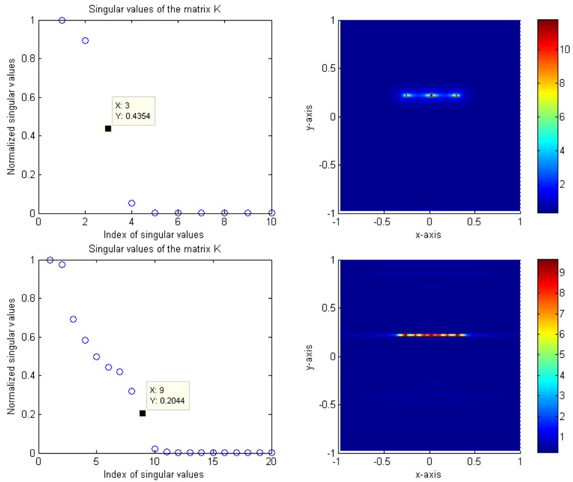
FIG. 2.2 – Distributions of normalized singular values of matrix K (left column) and maps of W_a(z) , z \in \tilde{\Omega} , a = 1 (right column), for N = 10 incidences and \lambda = 0.8 wavelength (top line), for N = 20 and \lambda = 0.2 (bottom line), when the inclusion is \Gamma_1 , with dielectric contrast of 5.
