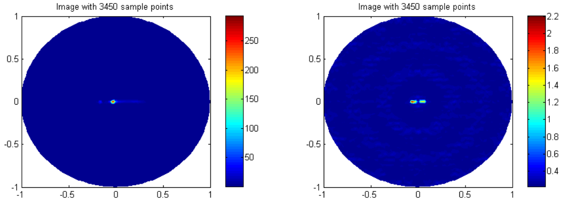
FIG. 5.11 – Left : image of \Sigma^{(3)} with the wavelength \lambda = 1 . Right : image of \Sigma^{(4)} with \lambda = 0.05 . The data set was generated by solving the forward problems.
