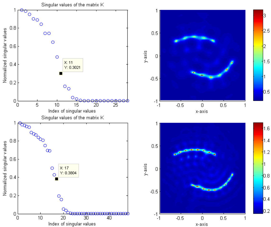
FIG. 4.12 – (Dirichlet boundary condition case) Distributions of normalized singular values of the matrix K (left column) and maps of W(z) (right column), for N = 28 incidences and a 0.5 wavelength (top line), for N = 48 incidences and a 0.3 wavelength (bottom line) when the crack is \Gamma_a .
