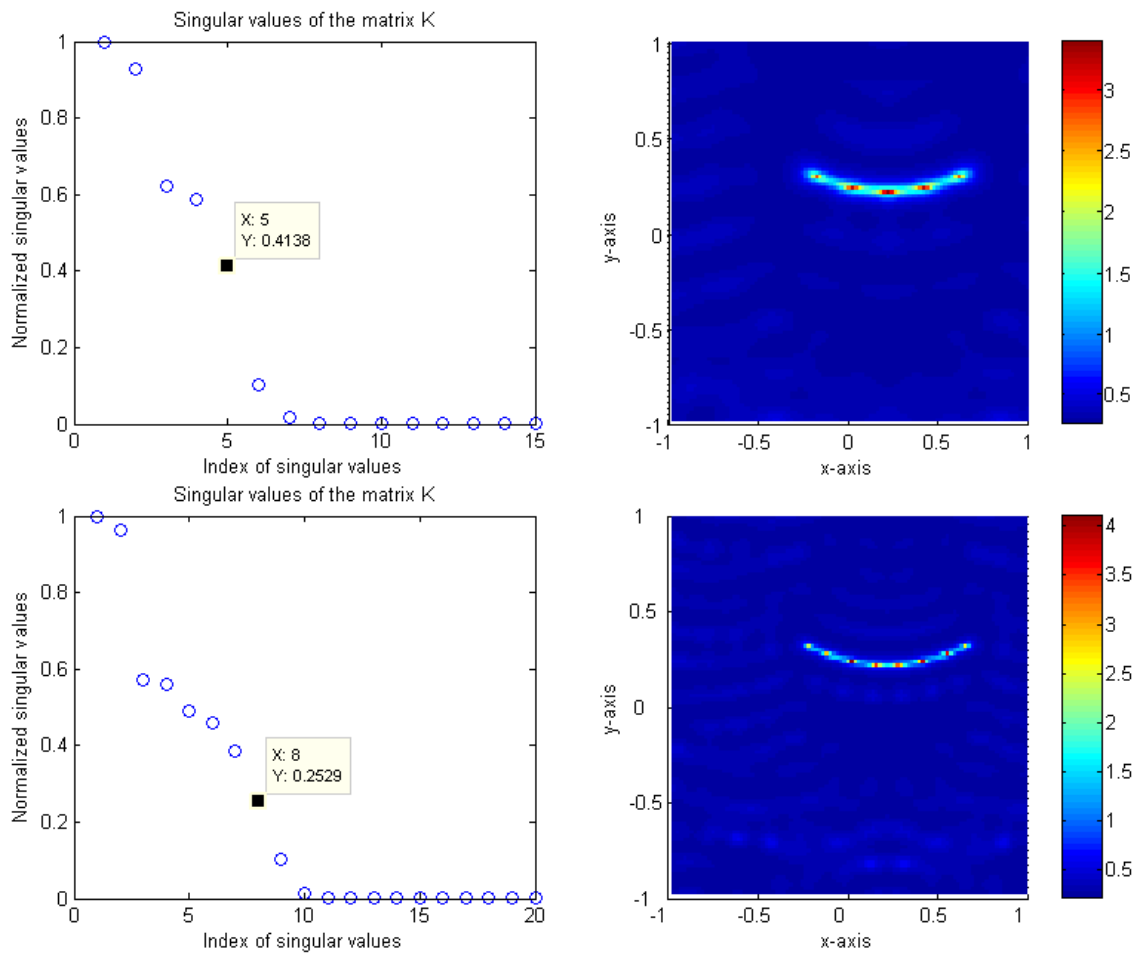
FIG. 2.5 – Distributions of normalized singular values of matrix K (left column) and maps of W_a(z) , z \in \tilde{\Omega} , a = 1 (right column), for N = 15 incidences and \lambda = 0.5 wavelength (top line), for N = 20 and \lambda = 0.3 (bottom line), when the inclusion is \Gamma_2 , with dielectric contrast of 5.
