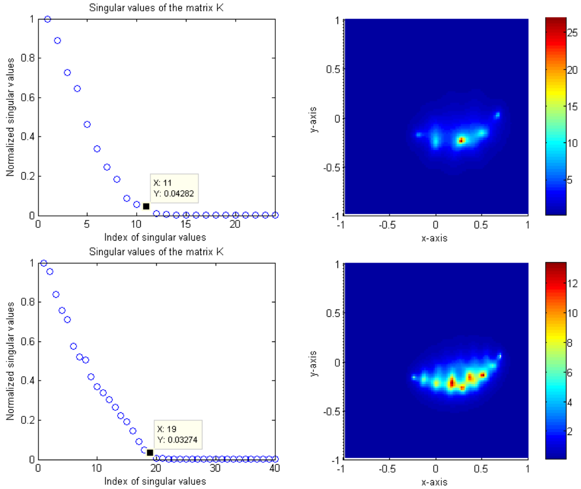
FIG. 2.25 – Distributions of normalized singular values of matrix K (left column) and maps of W_c(z) , z \in \tilde{\Omega} , c = (1, 0, 1) (right column), for N = 24 incidences and a \lambda = 0.6 wavelength, using 11 (top row) and 19 (bottom row) singular values for imaging, when the inclusion is \Gamma_3 , with dielectric and magnetic contrast of 5 each.
