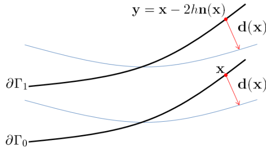
FIG. 3.5 – Deformation of a thin inclusion.
