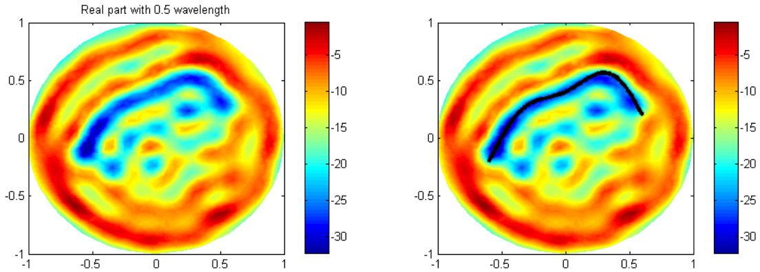
FIG. 5.13 – Image of d_T J(z) when \omega = \frac{2\pi}{0.5} , without noise
