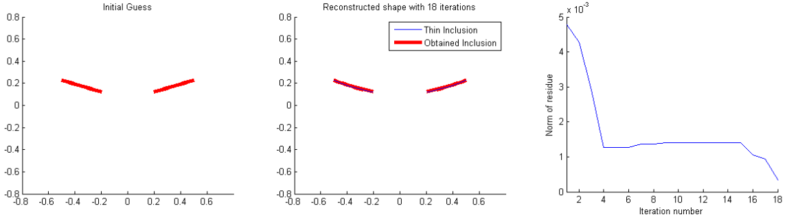
FIG. 3.16 – Reconstruction of \Gamma_3 for the permeability contrast case. From left to right initial guess, 18 iterations, true shape and normalized norm of data residuals for each iteration.
