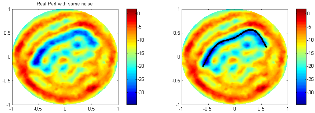
FIG. 5.14 – Image of d_T J(z) when \omega = \frac{2\pi}{0.5} , with noise \xi = 0.3 .
