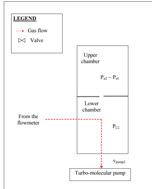
Figure 1.6. Valving sequence of the NIST primary standard for calibrating leak flow rate through the lower chamber: step 2.
