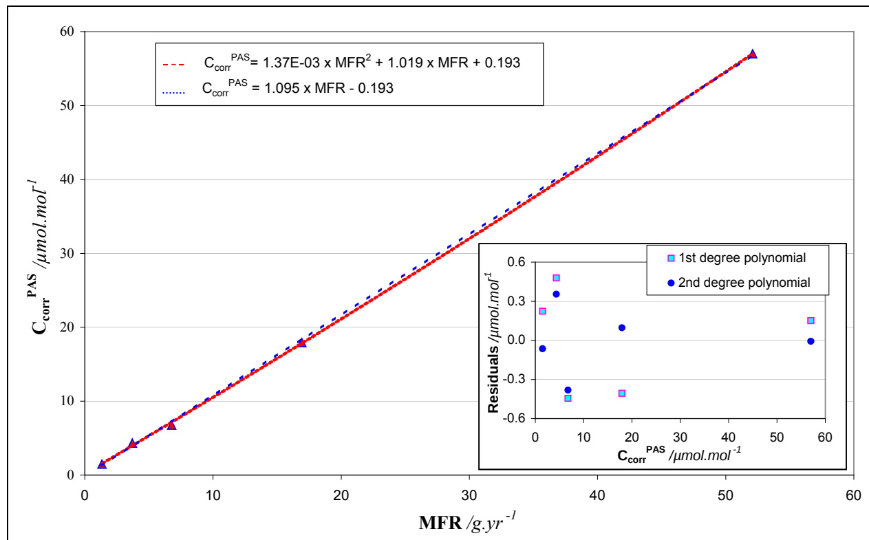
Figure 4.18. Example of a polynomial graph C_{corr}^{PAS} = f(\text{MFR}) , established according to Test 1 of the standard EN14624, and its associated residuals.
