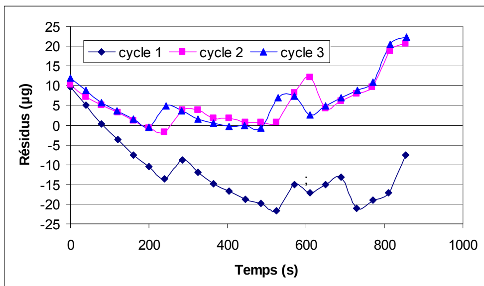
Figure 2.9. Residuals : fitting of the mass versus time considering all the cycles.
