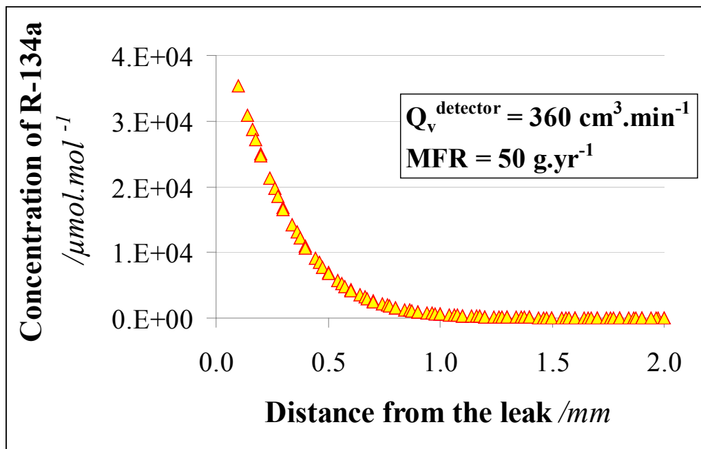
Figure 4.9. Changes of R-134a molar fraction in the cylindrical control volume as a function of coordinate x in the line ( x ; z = 0 ; y = 0 ), due to a 50 \text{ g.yr}^{-1} leak and to a 360 \text{ cm}^3.\text{min}^{-1} suction of the detector installed at 2 mm from the leak.
