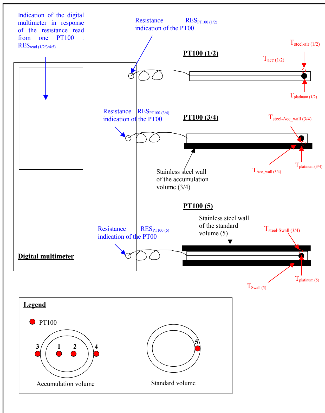
Figure 3.11. Diagram of the temperature measurement chain in the bench to calibrate refrigerant leaks.
