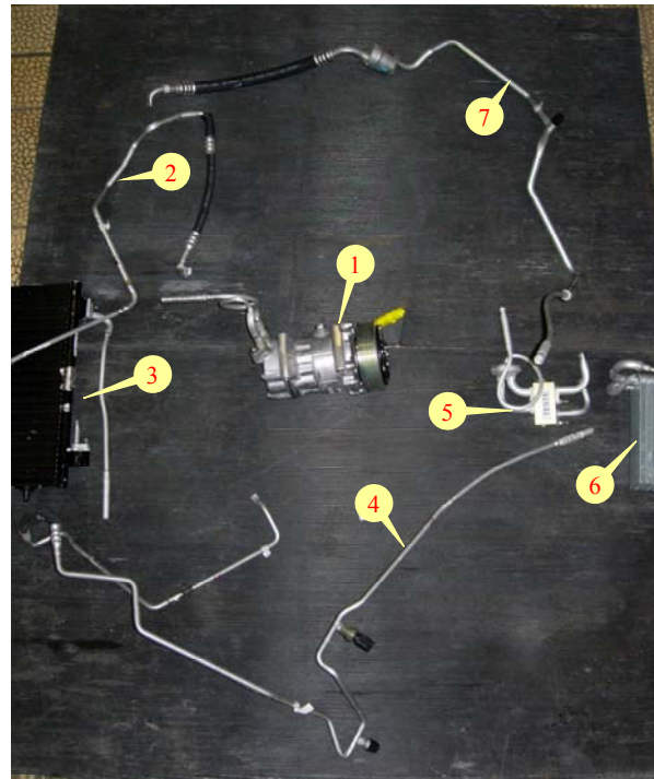
Figure 4.20. Example of a MAC system cut into parts [YU06].
