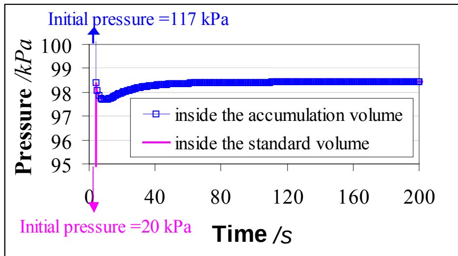
Figure 3.16. Simulation of an expansion from the accumulation volume to the standard volume: variation of pressures.
