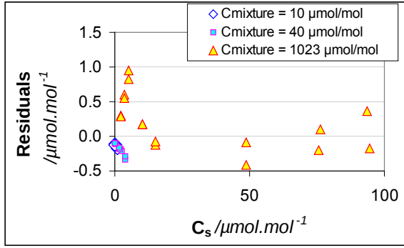
Figure 3.5. Residuals of a second order polynomial fitting of C_s = f(C_{\text{read}}) as a function of the diluted concentrations C_s made from the 3 standard mixtures ( 10.660 \pm 0.055 ) \mu\text{mol.mol}^{-1} , ( 42.40 \pm 0.10 ) \mu\text{mol.mol}^{-1} and ( 1023.5 \pm 5.2 ) \mu\text{mol.mol}^{-1} .
