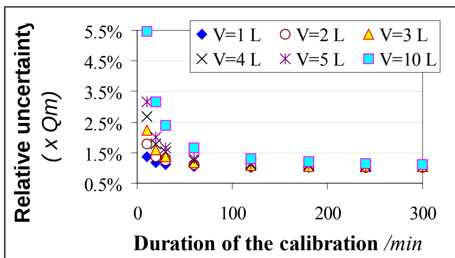
Figure 2.7. Theoretical relative uncertainty of the leak flow rate about 1 \text{ g.yr}^{-1} as a function of the duration of the calibration for different values of the capacity of the accumulation volume.
