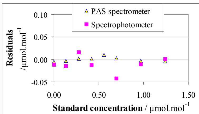
Figure 2.6. Residuals from a linear fitting relating the PAS and the spectrophotometer measurements of the standard concentrations (scale from 0.00 to 1.3 \mu\text{mol}\cdot\text{mol}^{-1} ) at 23^\circ\text{C} .
