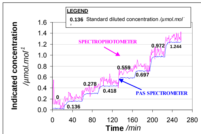
Figure 2.4. Measurements of a sample of standard concentrations of R-134a from 0 to 1.244 \mu\text{mol.mol}^{-1} at 23^\circ\text{C} .
