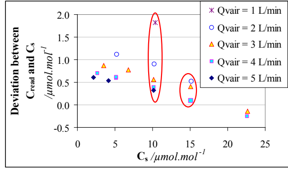
Figure 3.6. Deviation between the measurement of the spectrometer C_{\text{read}} and the diluted concentration C_s made from the standard mixture ( 1023.5 \pm 5.2 ) \mu\text{mol.mol}^{-1} with different ratios of gas/air volume flow rates, versus C_s .
