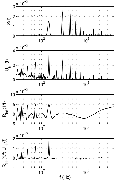
Fig. 2. From top to bottom, on a logarithmic frequency scale: parametric spectrum, spectral estimation function U_{\text{inh}}(f) , remapped temporal estimation function R_{\text{inh}}(\frac{1}{f}) , joint F_0 estimation function. Functions result from the 60 ms analysis of a D3 piano note.
