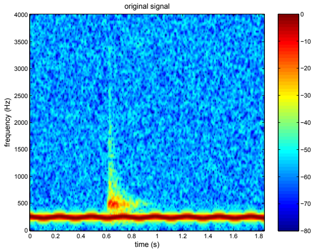
Fig. 7: Time-frequency representation of the original signal.
