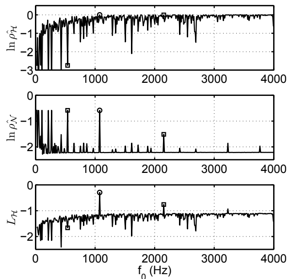
Figure 4: \mathcal{H} -dependent terms \ln \rho_{\mathcal{H}} (top) and \ln \rho_{\mathcal{N}} (middle), and weighted likelihood L_{\mathcal{H}} (bottom), computed for all possible F_0 's ( i.e. all possible \mathcal{H} 's).
