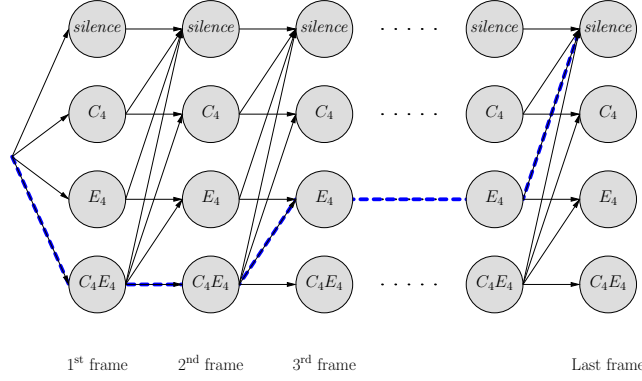
Figure 1: Chord network corresponding to the transition matrix of Table 1. Due to the sparsity of the transition matrix, transitions are allowed toward the same chord or toward a "subchord", when note endings occur. The thick, dashed line shows a possible Viterbi path: chord \{C_4, E_4\} is detected, C_4 dies at frame 3 while E_4 lasts until next to last frame of the segment.
