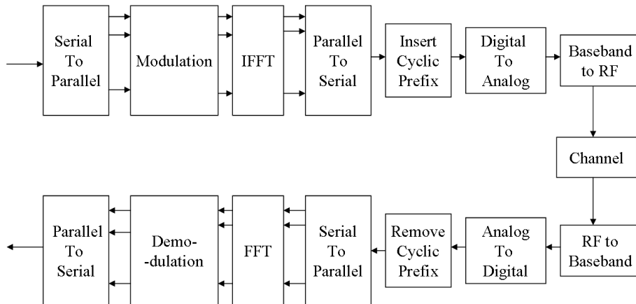
Figure 2.1: Implementation of an OFDM system
