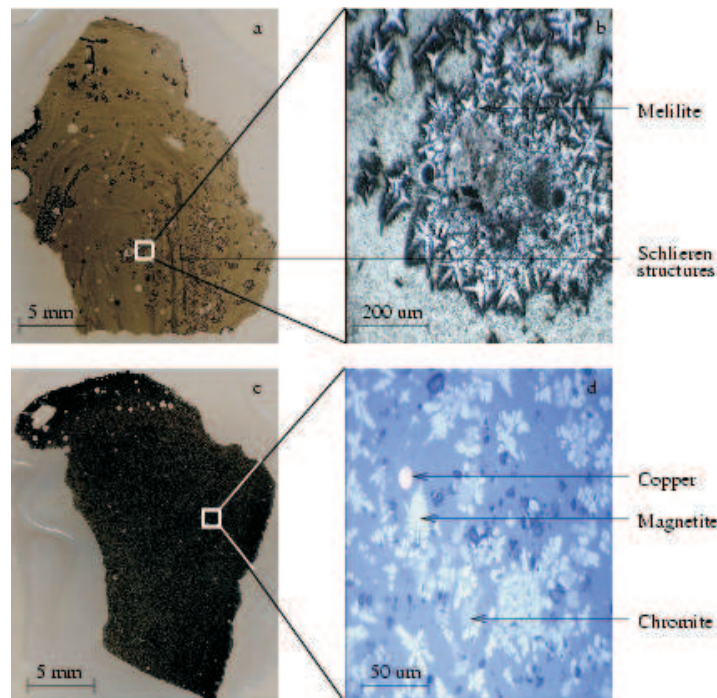
FIG 2 - Examples of primary glassy phases present in MSWI bottom ash: (A) primary melilite-bearing glass with (B) detailed zoom in transmitted light microscopy; (C) opaque glass with (D) detailed zoom in reflected light microscopy (minerals determined by SEM-EDS).
