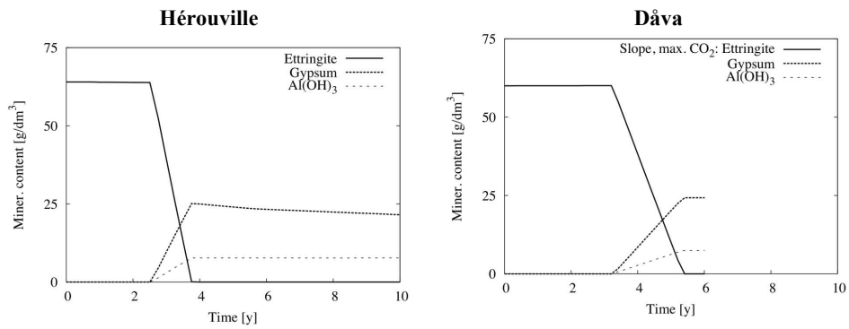
Fig. 6. Transformation of ettringite into calcite (not shown, see Fig. 4), gypsum and aluminum hydroxide in the MSWI bottom ashes, located close to the sampling point at Hérouville and in the slope sampling point at Dåva in the case of the maximum CO 2 input.
