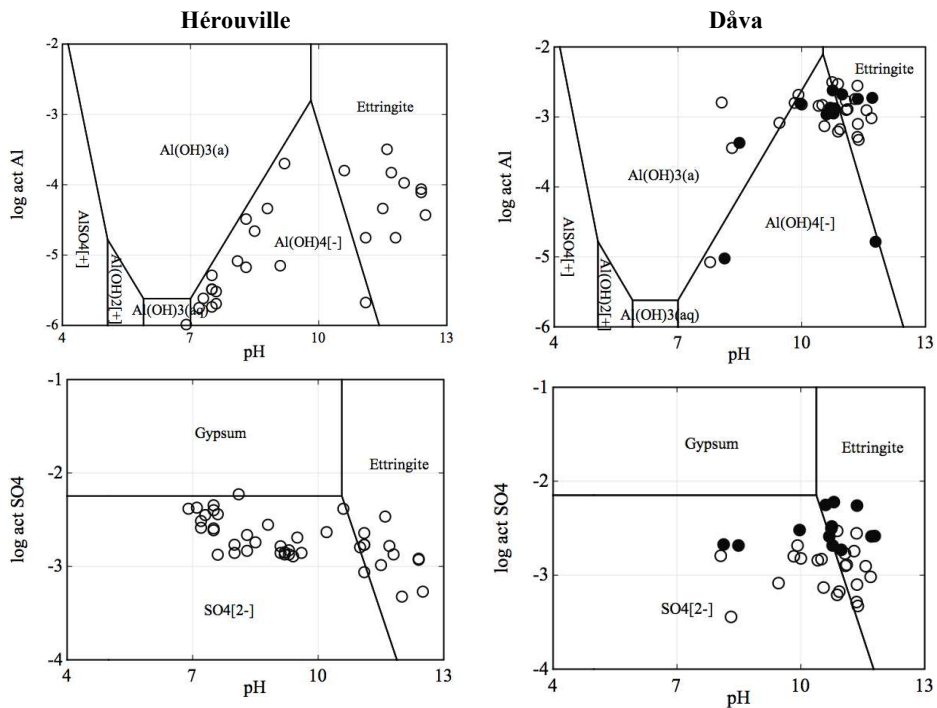
Fig. 7. Plot of the leachate experimental data on aluminum and sulfate solubility diagrams for the two test roads (in the Dåva case, the symbols \circ and \bullet stand for the lysimeter under the slope and the road, respectively).
