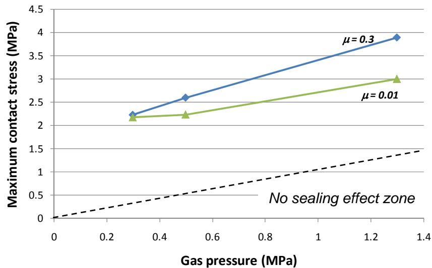
Figure 4-7 Rubber lip edge contact stress evolution with fluid pressure and friction coefficient.
