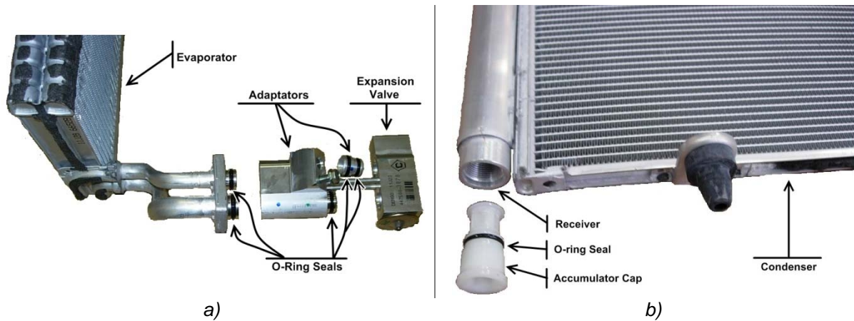
Figure 1-6 Examples of heat exchangers and expansion device sealing system.
