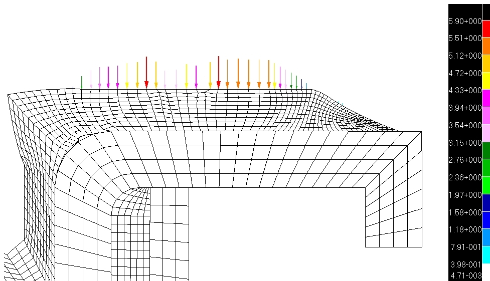
Figure 4-4 Peripheral rides deformation and contact stress distribution, P=0.3 MPa and \mu=0.3 .
