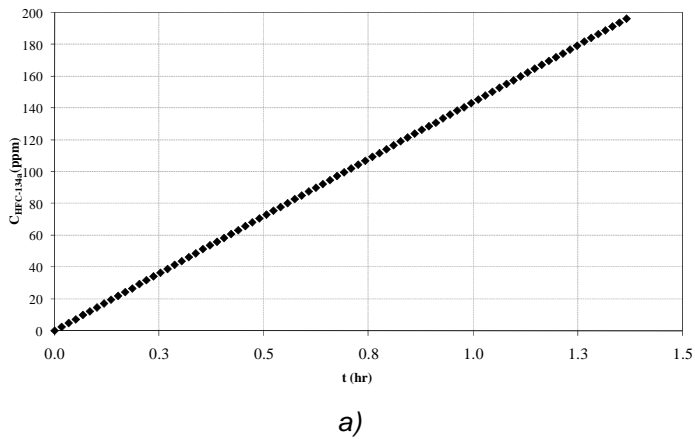
Figure 2-20 Evolution of the gas concentration in the accumulation volume a) using a calibrated leak b).
