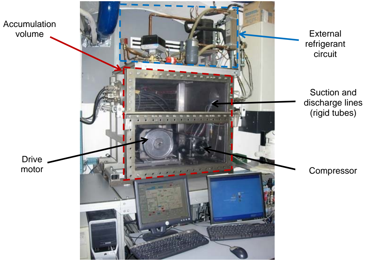
Figure 2-17 Picture of the experimental setup.
