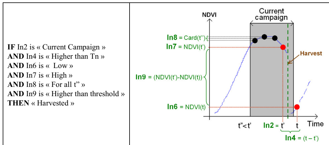
Figure 7. An example of a rule generated automatically using learning data, with a schematisation of the scenario that it reflects. The rule is defined using a subset of input variables (In1, ..., In11) and a conclusion. Each point in the NDVI temporal profile represents the NDVI value of the sugarcane field calculated at a given acquisition date ( t , t' or t'' < t' ).
