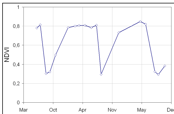
Figure 2. Example of the temporal profile of sugarcane NDVI calculated for a ratoon crop.
