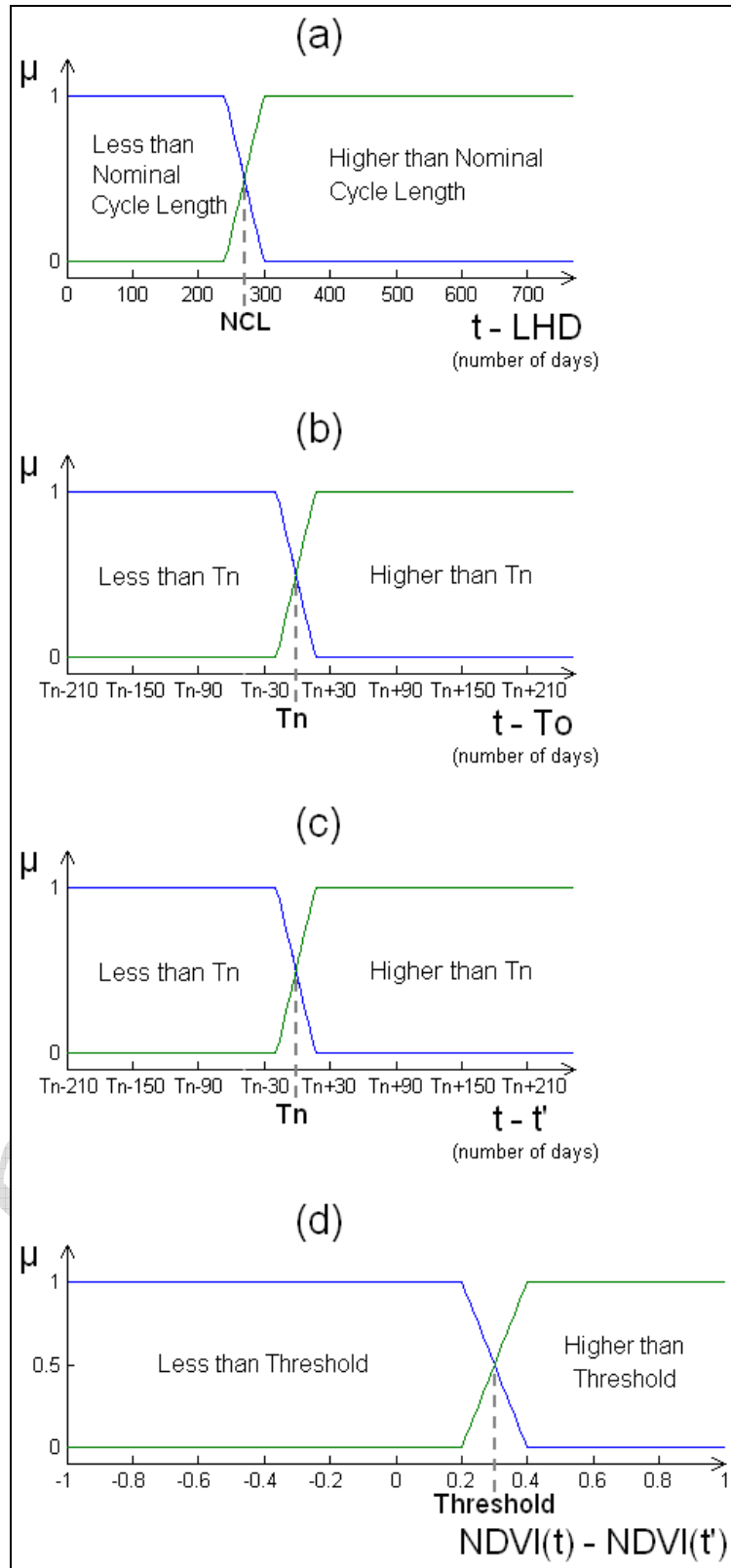
Figure 7: Fuzzy sets of inputs In3 (a), In4 (b), In5 (c) and In9 (d). LHD = Last harvest date, NCL = Nominal cycle length, T_n = Nominal time, T_0 = opening mill date, and Threshold = \Delta \text{NDVI}_{\text{Threshold}} .
